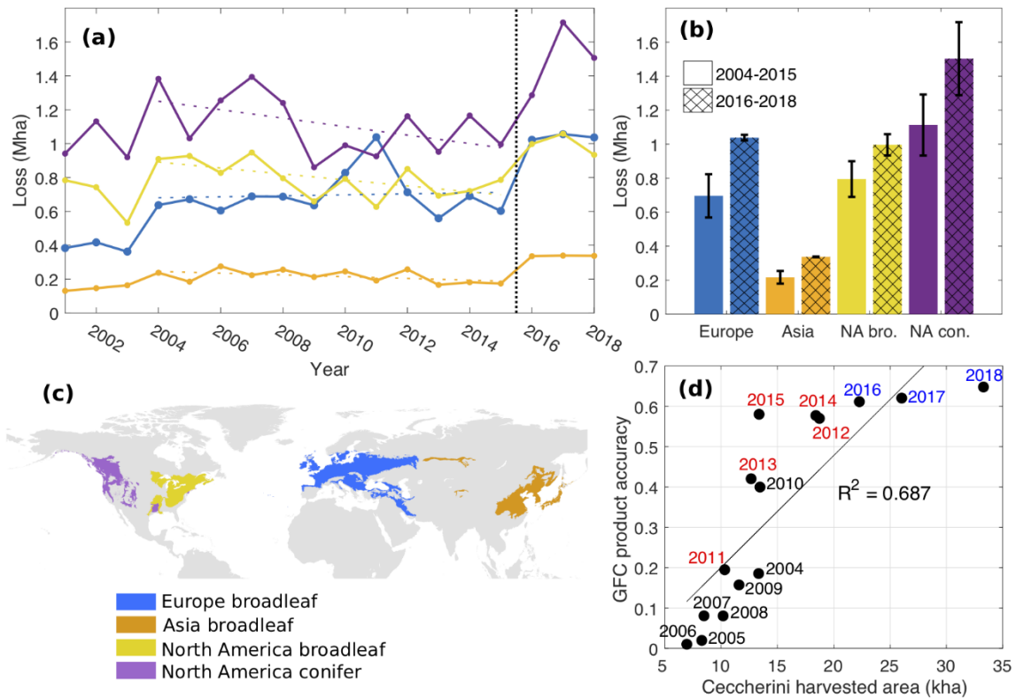
Fig. 1 | Abrupt changes in GFC after 2015 are visible in many temperate regions. This reflects the various improvements in detection that were noted in ref. 4 . a , Annual forest cover loss from GFC data in four forest regions: Europe broadleaf (blue); Asia broadleaf (orange); North America broadleaf (yellow) and North America conifer (purple). The vertical dashed line marks the point of the increase in loss reported by Ceccherini et al. 1 . Dashed coloured lines are linear regressions over the period 2004–2015. b , The mean annual loss over 2004–2015 and 2016–2018; error bars show \pm 1 s.d. (sample size is number of years each). c , The locations of the four forest regions. d , A comparison between the harvested area proposed by Ceccherini et al. 1 for Italy and the accuracy of the GFC forest loss as measured in ref. 5 (based on comparison against harvested areas mapped in the field). The increase in estimated harvest from the GFC largely reflects changes in detection. Different colours denote the periods compared by Ceccherini et al. 1 .
