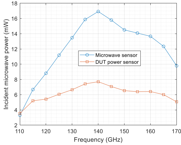
Fig. 5. Incident microwave power on the microwave sensor and on the DUT power sensor.
