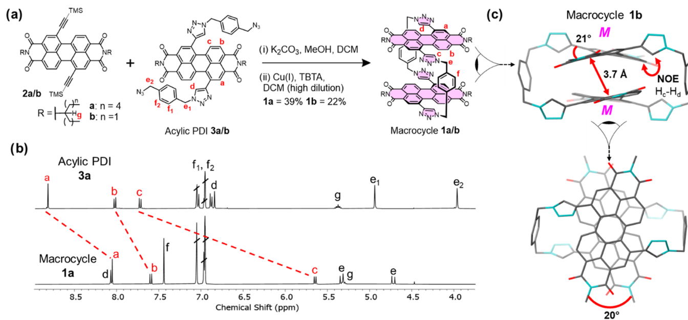
Figure 2. (a) Synthesis of bis-PDI macrocycles 1a/b. (b) Comparison of the ^1\text{H} NMR spectra of macrocycle 1a and acyclic PDI 3a (toluene- d_8 , 373 K, 400 MHz). (c) X-ray crystal structure of macrocycle 1b ( MM ), viewed from the side and the top (alkyl side chains, hydrogens, and cocrystallized solvent molecules are omitted for clarity, see the Supporting Information, Section 3).
