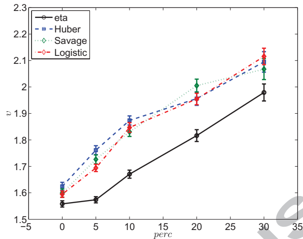
Figure 6: Performance of twin boosting algorithms with robust eta (RTBFS), Huber, Savage and standard Logistic loss functions (STBL) in terms of the average proportional increase in error ( \nu ) for 5NN. perc is the percentage of contamination.
