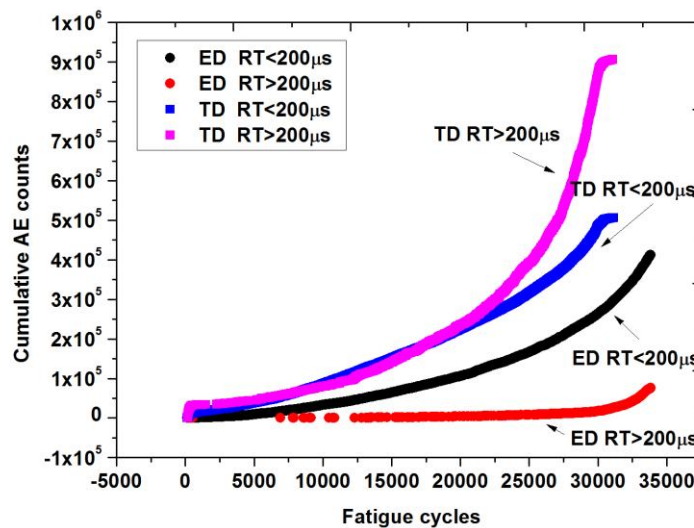
Fig. 11 Cumulative AE counts for AE events with RT < 200\mu s and RT > 200\mu s in ED and TD specimens during FCP
