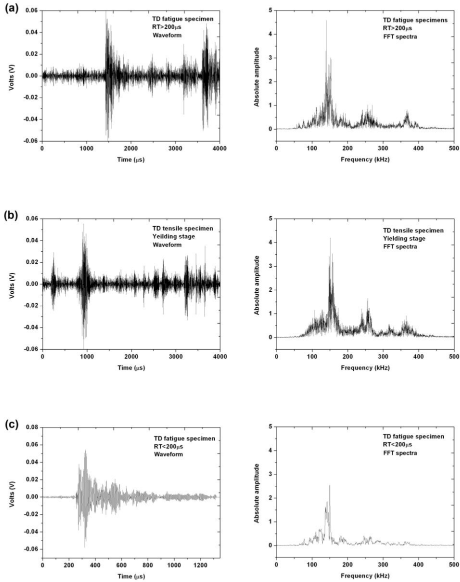
Fig. 10 Typical waveforms and FFT spectrum for (a) signals with higher RT (>200μs) during fatigue test for TD specimen (b) signals in yielding stage during tensile test for TD specimen (c) signals with lower RT (<200μs) during fatigue test for TD specimen
