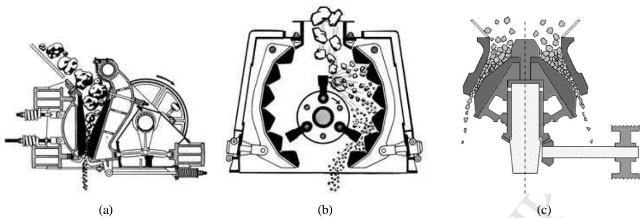
Figure 8 - Examples of (a) a jaw crusher (b) an impact crusher and (c) a cone crusher (Crushersale, 2013; Penncrusher, 2013)
