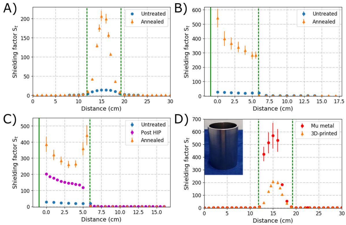
Figure 4. Measured shielding factors along the test and control shields longitudinal axes, under an external magnetic field of 50 \mu\text{T} . The dashed lines show the position of the open ends of the shields, while the solid lines shows the closed ends. A) Open ended test shield B) Closed ended test shield C) Closed ended test shield which underwent HIP treatment. The increase in shielding factor towards the open end of the test shield has been seen in 3D-printed shields that have not received the HIP treatment and therefore is not an effect of the HIP treatment. D) Comparison of the open ended test shield and the control shield. The inserted image shows the replica mu-metal shield. The mu-metal replica was annealed in pure dry hydrogen under the same conditions as the 3D-printed samples. The maximum magnetic shielding factor measured in the control shield was 568 \pm 102 .
