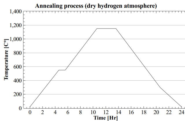
Figure 10. Annealing treatment cycle in pure hydrogen atmosphere used for all the 3D-printed magnetic shield samples and mu metal shield.
