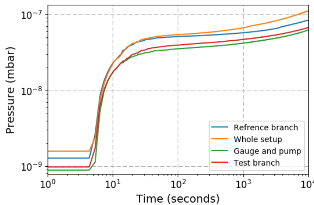
Figure 8. Rate of rise curves for the different sections of the vacuum system. The pressure before the rate of rise curve is not representative of the minimum achievable pressures but instead of the pressure in the chamber before the test was carried out.
