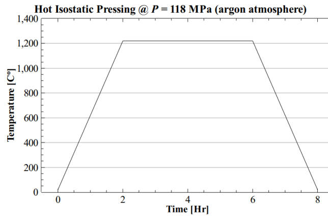
Figure 9. Hot isostatic pressing process cycle in argon atmosphere used for the 3D-printed sample in figure 4 D.
