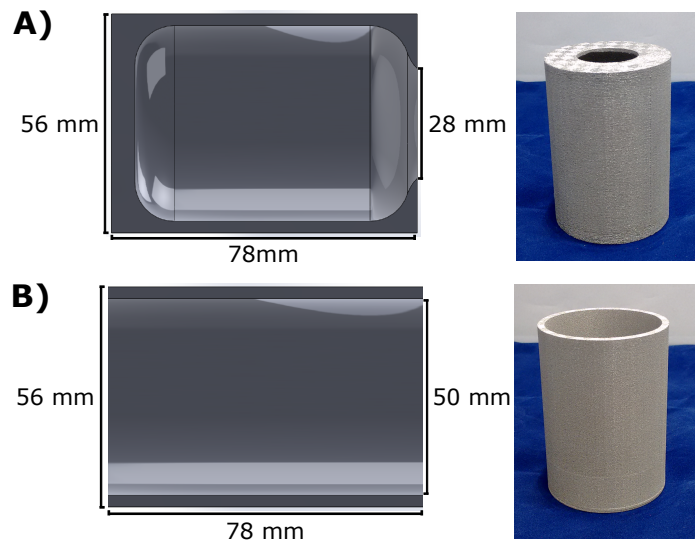
Figure 1. The 3D-printed magnetic shield structures used as test pieces. A) Closed ended magnetic shield dimensions and a photo of the 3D-printed structure. B) Open ended magnetic shield dimensions and a photo of the 3D-printed structure.
