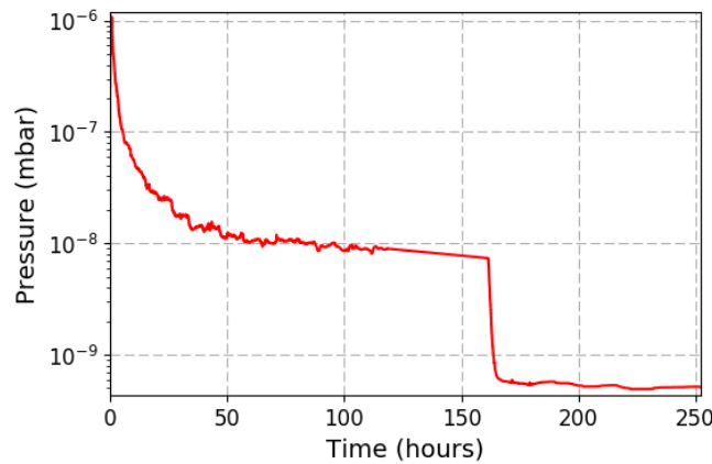
Figure 7. Chamber pressure of the entire system vs time, after equalisation at a bake-out temperature of \sim 130^{\circ}\text{C} . After 160 hours the bake out ended and the temperature of the system returned to room temperature ( \sim 21^{\circ}\text{C} ), and the pressure in the chamber reduced by roughly an order of magnitude.
