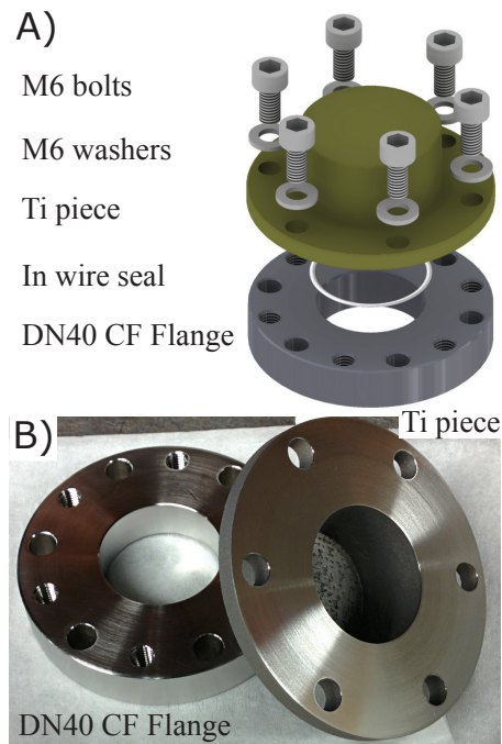
Figure 5. A) Digital render of the vacuum flange structure with components for vacuum sealing. The test piece was designed with a top hat profile with a diameter of 70mm and indium sealed onto a stainless steel flange. The stainless steel flange had bore holes of 30mm and 6 M6 tapped holes to apply pressure to the indium seal. Once sealed the DN40CF flange is attached to the chamber using a standard copper gasket. The holes in test piece the are compatible with a DN40CF flange. B) The DN40 CF flange and test piece prior to Assembly.
