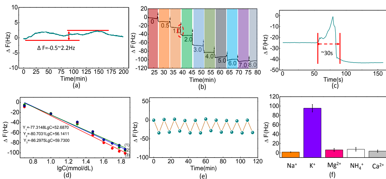
Figure 4. The sensitivity, reusability, and selectivity of 18-crown-6 ether functionalized hydrogels films based on a QCM sensor to identify \text{K}^+ ions. (a) Frequency shift over 200 min in 3 mM KCl solution. (b) The 18-crown-6-ether functionalized hydrogel film coated on a QCM chip in response to various KCl concentrations. (c) Enlarged image of the red area (b). (d) Fitted curve depicting the change in frequency shift and the logarithm of KCl concentration. (e) Reversibility of the 18-crown-6 ether functionalized hydrogel films coated on a QCM chip. (f) Comparison of the resonance frequency shift of the 18-crown-6 ether functionalized hydrogel films to 6.0 mM solutions of different monovalent and divalent metal ion solutions.
