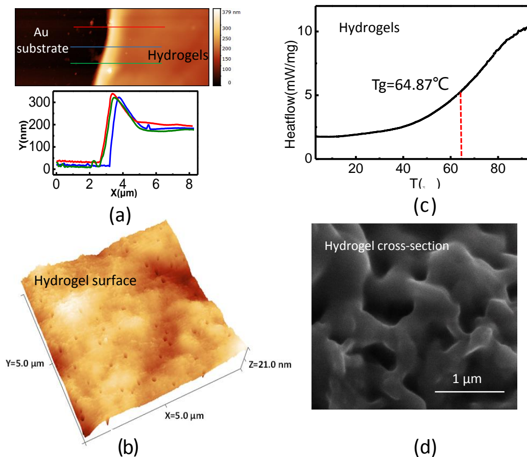
Figure 2. The homogeneity, mechanical properties, and morphology of the hydrogel film. (a) Thickness of the hydrogel thin film. (b) AFM image of the hydrogel surface morphology. (c) DSC curves of the hydrogels. (d) SEM image of the hydrogel's cross-section morphology.
