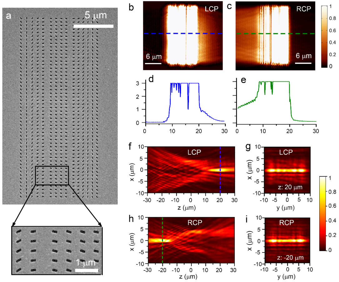
Figure 3| Experimental results of the optical performances in the near and far fields for the 2D metasurface. (a) Scanning electron microscopy (SEM) images of the fabricated 2D metasurface. (b, c) Measured optical near-field intensities with (b) LCP and (c) RCP incidences. (d, e) Line-cut of intensities versus x -coordinate for the dashed lines in b, c. (f, g) Measured optical far-field intensities at (f) xz plane and (g) real focal xy plane ( z=20\ \mu\text{m} ) with LCP incidence. (h, i) Measured optical far-field intensities at (h) xz plane and (i) virtual focal xy plane ( z=-20\ \mu\text{m} ) with RCP incidence.
