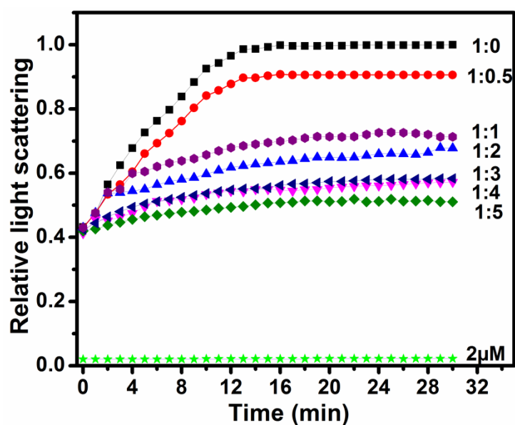
Fig. S4. Prevention of thermal aggregation of MalZ by minichaperone. 0.5µM MalZ was incubated at 50°C in the absence or presence of increasing amounts of minichaperone as indicated. The molar ratio of MalZ and minichaperone is indicated against each aggregation trace. Aggregation kinetics was monitored by light scattering at 500nm and normalized to the value of MalZ aggregation in the absence of minichaperone. The green star trace shows that minichaperone alone does not aggregate at 50°C.
