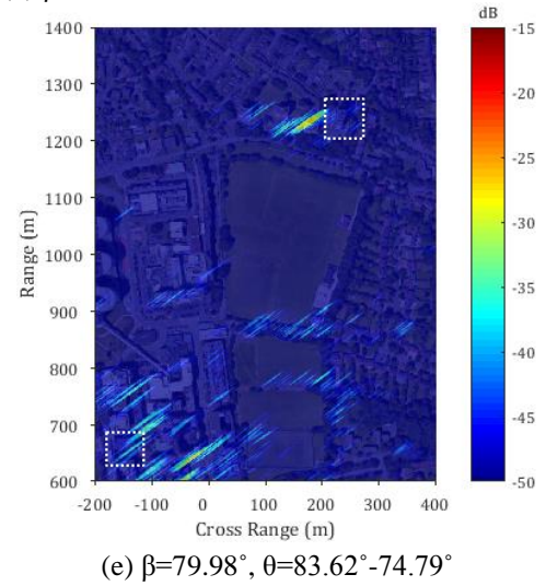
Figure 7: Example bistatic images obtained from (a) Galileo GSAT-0205-24 E5a, (b) GPS BIIF-05-30 L5, (c) Galileo GSAT-0214-05 E5a, and (d)-(e) GPS BIIF-07-09 L5
