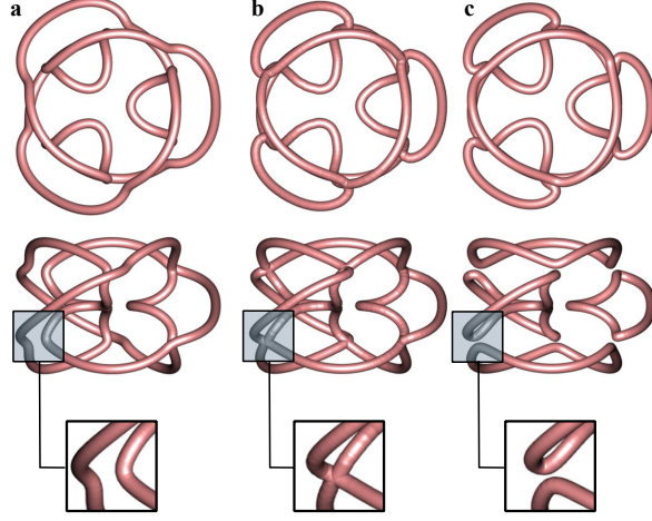
Fig. 4. Reconnection events destroying vortex knot in E_- component. The parameter s is decreased from (a) s = 1.000 , where there is a knotted vortex line, through the critical value of s_c = 0.965 where the vortices touch at six points. At lower values of s , such as (c) s = 0.950 , the vortex configuration is five unlinked rings. In each frame, there is an axial view, a side view and an inset showing the vortex geometry.
