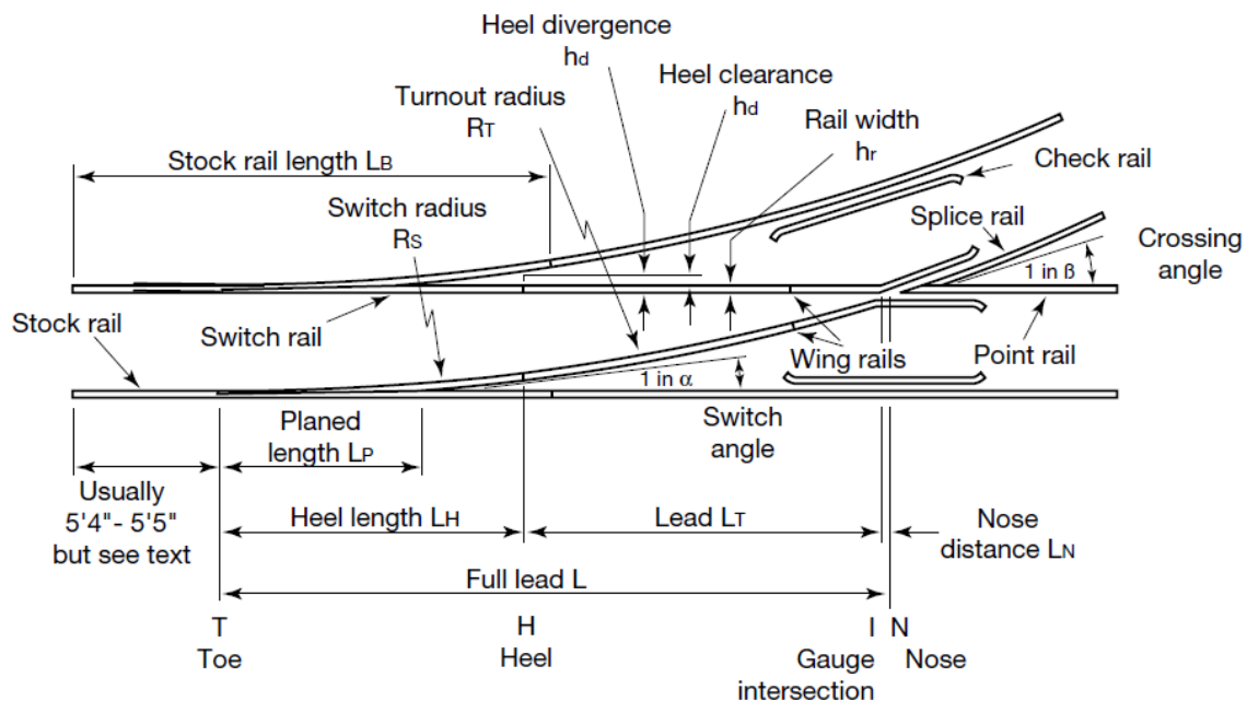
Figure 3: The geometry of a turnout (Gauge O Guild, 2004)
