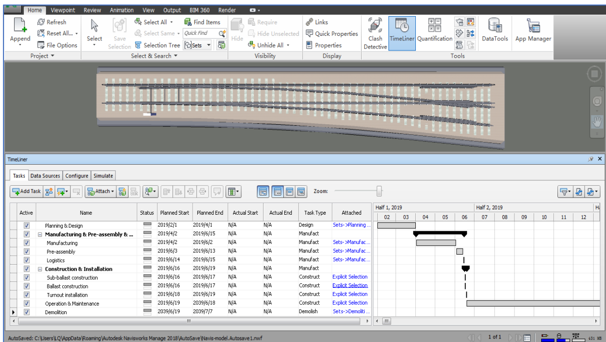
Figure 10: 4D simulation of turnout system in Navisworks-2018
