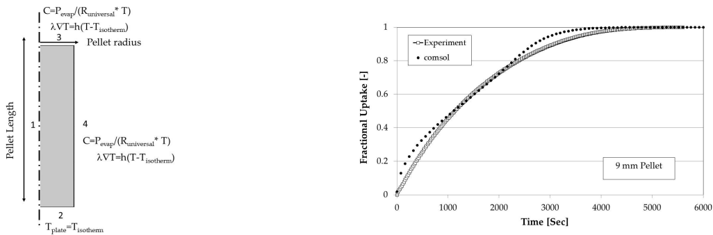
Fig .2. (a) Model boundary conditions (b) Model validation
