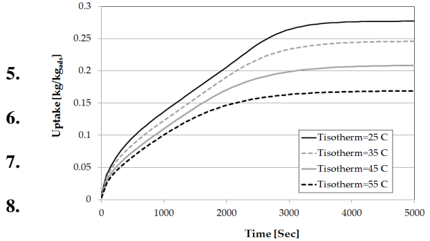
(b) Effect of adsorption temperature
