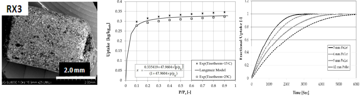
Fig. 1. (a) SEM of 3 mm of RX3 (b) Langmuir isotherm model (c) Fractional uptake of different pellets
