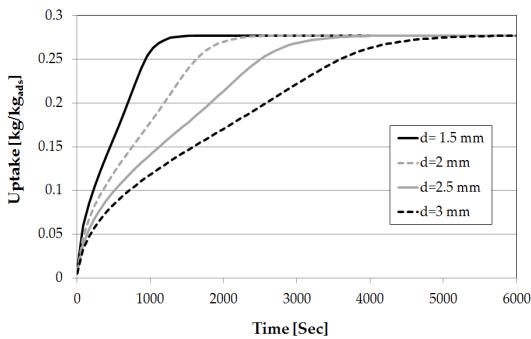
Fig. 4. (a) Effect of pellet diameter
