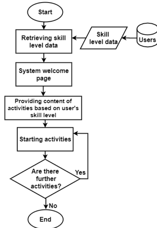
Figure 2: The proposed content matching algorithm based upon reading skill level.
