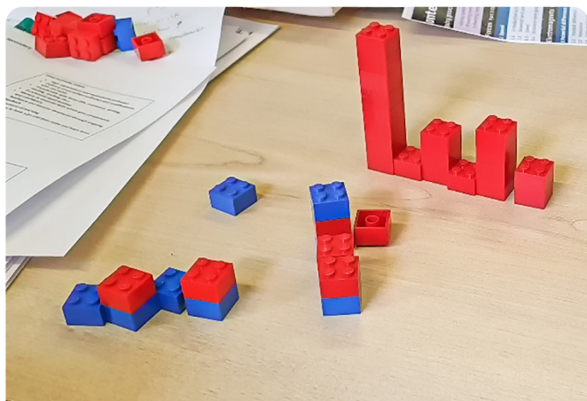
Figure LEGO used to represent a bar chart
