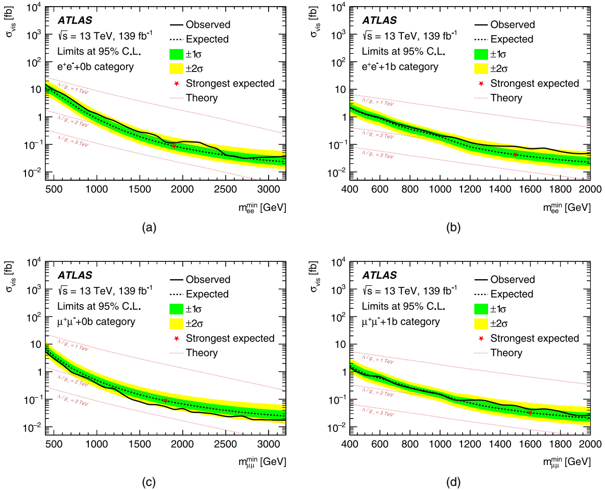
FIG. 4. Model-independent observed (solid line) and expected (dashed line) upper limit on the visible cross section ( \sigma_{\text{vis}} = \sigma\epsilon\mathcal{A} ) for the (a) electron b -veto, (b) electron b -tag, (c) muon b -veto, and (d) muon b -tag categories. The uncertainty bands around the expected limit represent the 68% and 95% confidence intervals. The theory lines (dotted lines) correspond to particular \Lambda/g_* values of the signal model, and the red marker presents the strongest expected lower limit on \Lambda/g_* .
