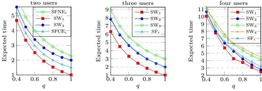
Fig. 2: Aloha: \langle\langle usr_1 : \dots : usr_m \rangle\rangle(\star_1, \star_2)_{\min} = ? (\mathbf{R}^{time}[\mathbf{F} \ s_1] + \dots + \mathbf{R}^{time}[\mathbf{F} \ s_m])
