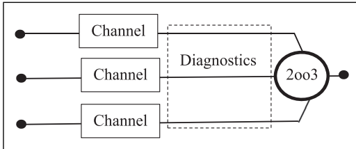
Figure 2. Two out of 3 voting architecture (Diagram from IEC61508 part 6).
