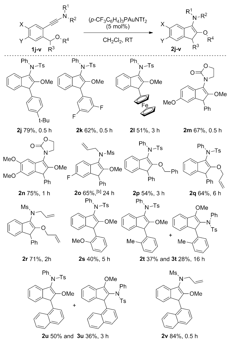
Scheme 3. Reaction scope. [a] Reaction conditions: 1 (0.2 mmol, 1 equiv), was reacted with (\text{p-CF}_3\text{C}_6\text{H}_4)_3\text{PAuNTf}_2 (5 mol%) in \text{CH}_2\text{Cl}_2 (0.1 M) at RT, time as indicated. [b] Using 10 mol% catalyst. Regioisomer 3o also isolated in a 10% yield.
