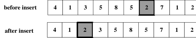
Fig. 7 Insert operator ( N_2 )
