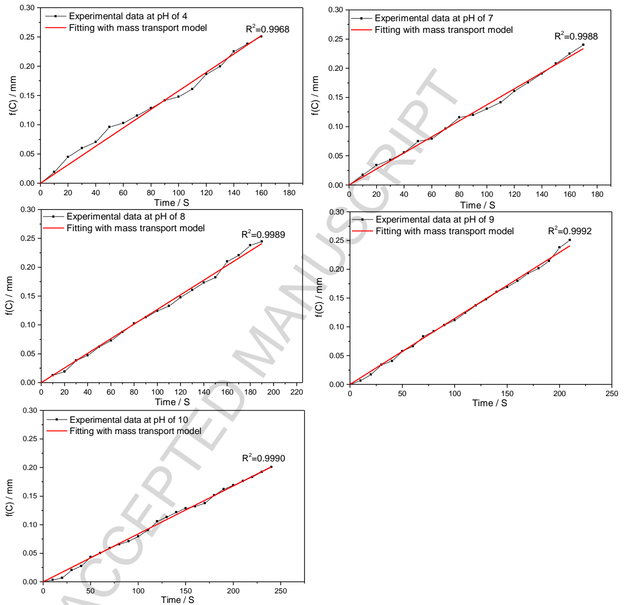
Fig.11. Fitting with mass transport model for the dissolution experiment at pH 4 / 7 / 8 / 9 / 10
