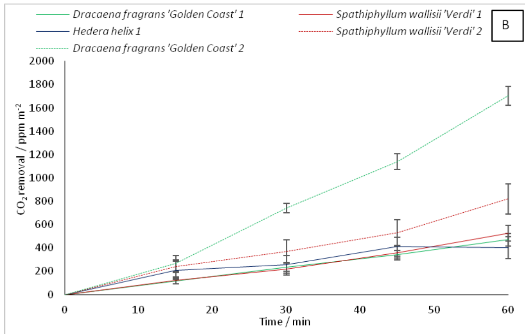
2 Figure 2: Mean CO 2 removal by each taxon in substrates 1 and 2 at 'very high' indoor light (~ 22000 lux, ~ 300 μmol 3 m -2 s -1 ) per m 2 of leaf area in 'wet' (SMC > 30 %, 0.3 m 3 m -3 ) (A), and 'dry' (SMC < 20 %, 0.20 m 3 m -3 ) (B) conditions 4 over a 60 min period. Data are a mean of five plants per taxa – error bars represent SEM.
