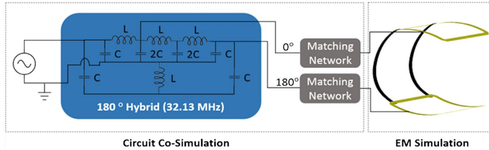
FIGURE 1 Schematic of the simulated model of the clamshell-type transmit coil with the hybrid circuit needed to excite the homogenous mode ( C = 140 pF, L = 350 nH)
