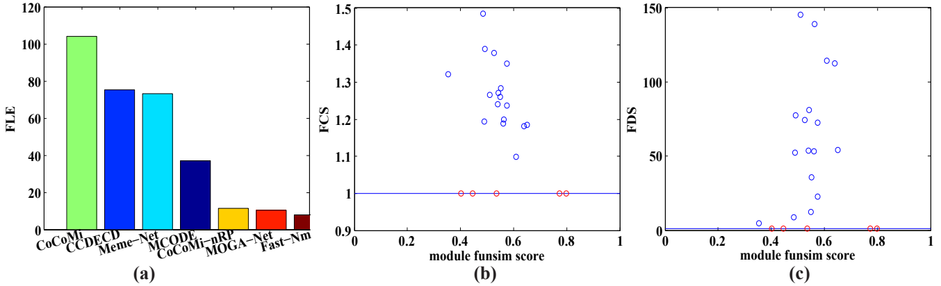
Fig. 10. (a) The FLE scores of partitions of modules obtained by the CoCoMi, CoCoMi-nRP and other algorithms on the GGPI network. (b) The FCS of modules of CoCoMi-nRP on the GGPI network. (c) The FDS of modules of CoCoMi-nRP on the GGPI network. Red circles indicate modules that cannot be no further partitioned by the RP scheme in CoCoMi.
