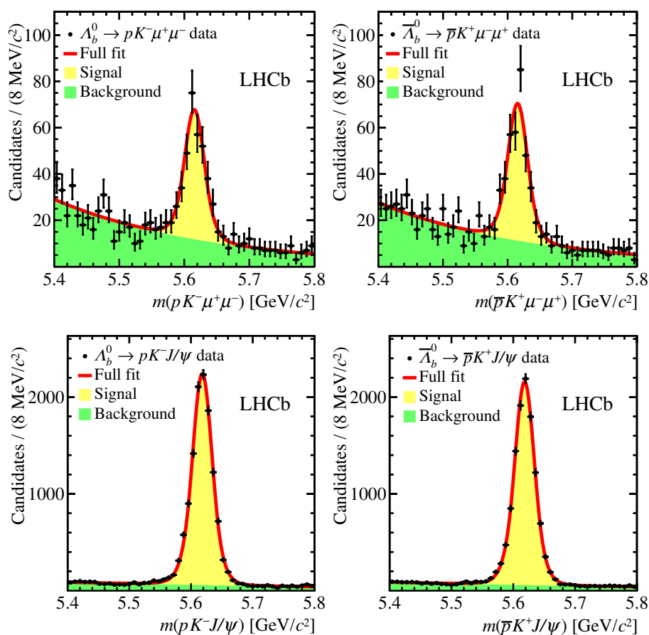
Figure 3. Invariant mass distributions of (top) \Lambda_b^0 \rightarrow pK^- \mu^+ \mu^- and (bottom) \Lambda_b^0 \rightarrow pK^- J/\psi candidates, with fit results superimposed. Plots refer to the (left) \Lambda_b^0 and (right) \bar{\Lambda}_b^0 subsamples.
