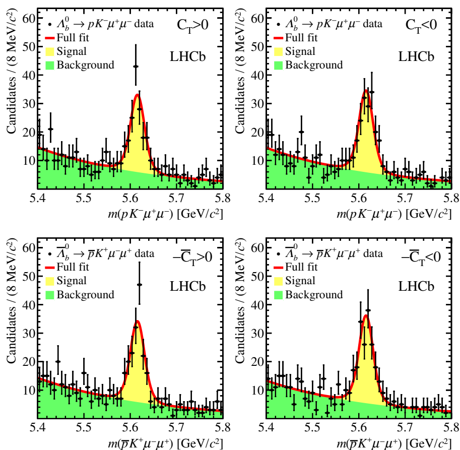
Figure 4. Invariant mass distributions of the \Lambda_b^0 \rightarrow pK^- \mu^+ \mu^- subsamples used for the A_{\hat{T}} and \bar{A}_{\hat{T}} measurements. Plots refer to (top) \Lambda_b^0 and (bottom) \bar{\Lambda}_b^0 decays divided into the subsamples (left) C_{\hat{T}} > 0, -\bar{C}_{\hat{T}} > 0 and (right) C_{\hat{T}} < 0, -\bar{C}_{\hat{T}} < 0 .
