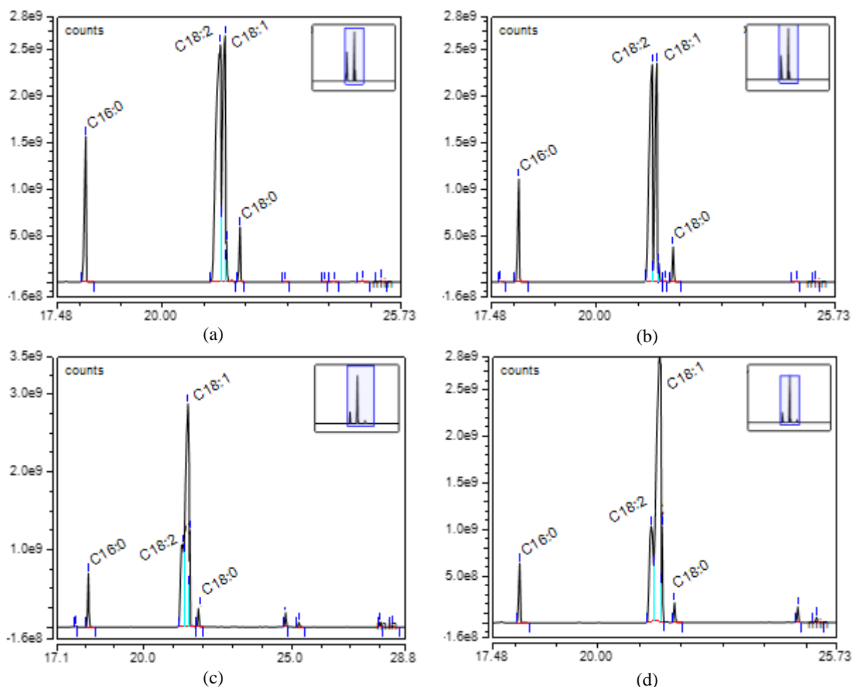
343 Fig. 4. Gas chromatography and mass spectrum analyse of (a) W100, (b) W85, (c) R100 and (d) R85.
