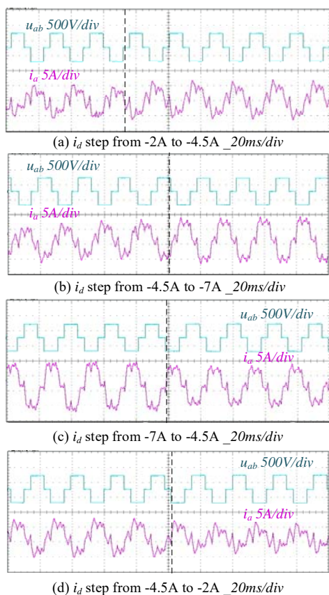
Fig. 18. Line voltage and phase current of current step response in six-step operation
