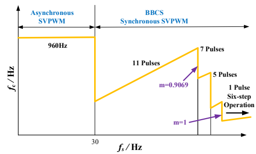
Fig. 13. PWM scheme of the inverter
