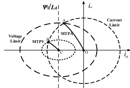
Fig. 4. Working areas of PMSM
