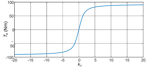
Fig. 9. The relation between torque and k_u
