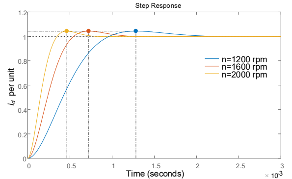
Fig. 10. The step response of the design with different motor speed
