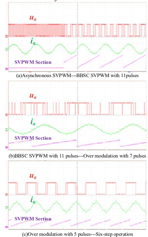
Fig. 14. PWM in full speed range
