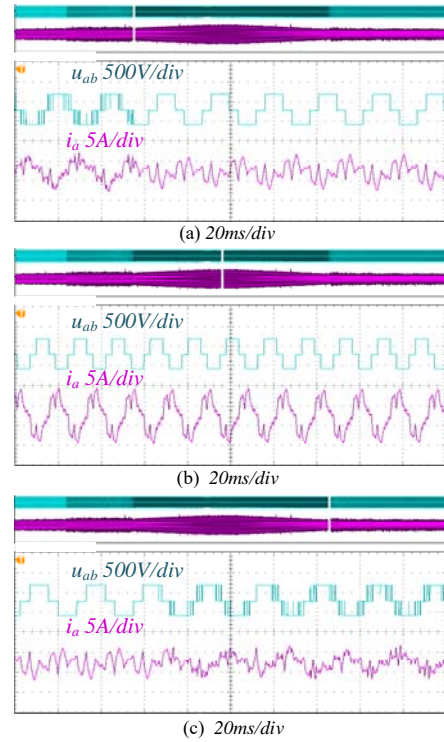
Fig. 16. Line voltage and phase current of speed closed-loop control
