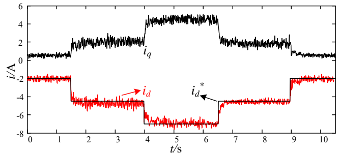
Fig. 17. Step response in six-step operation
