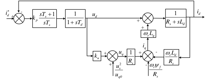
Fig. 7. Converted control block diagram
