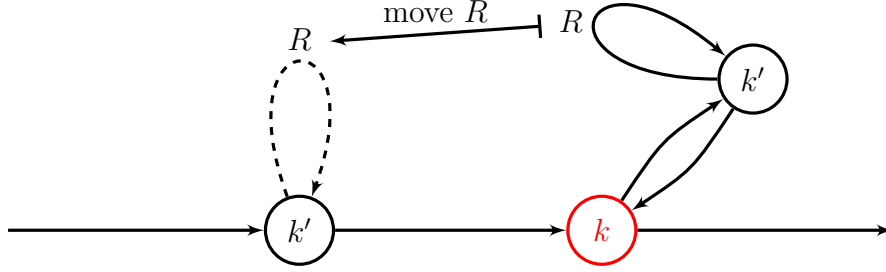
Figure 7: Node k' appears twice in C_1 = kP_1V_1k
