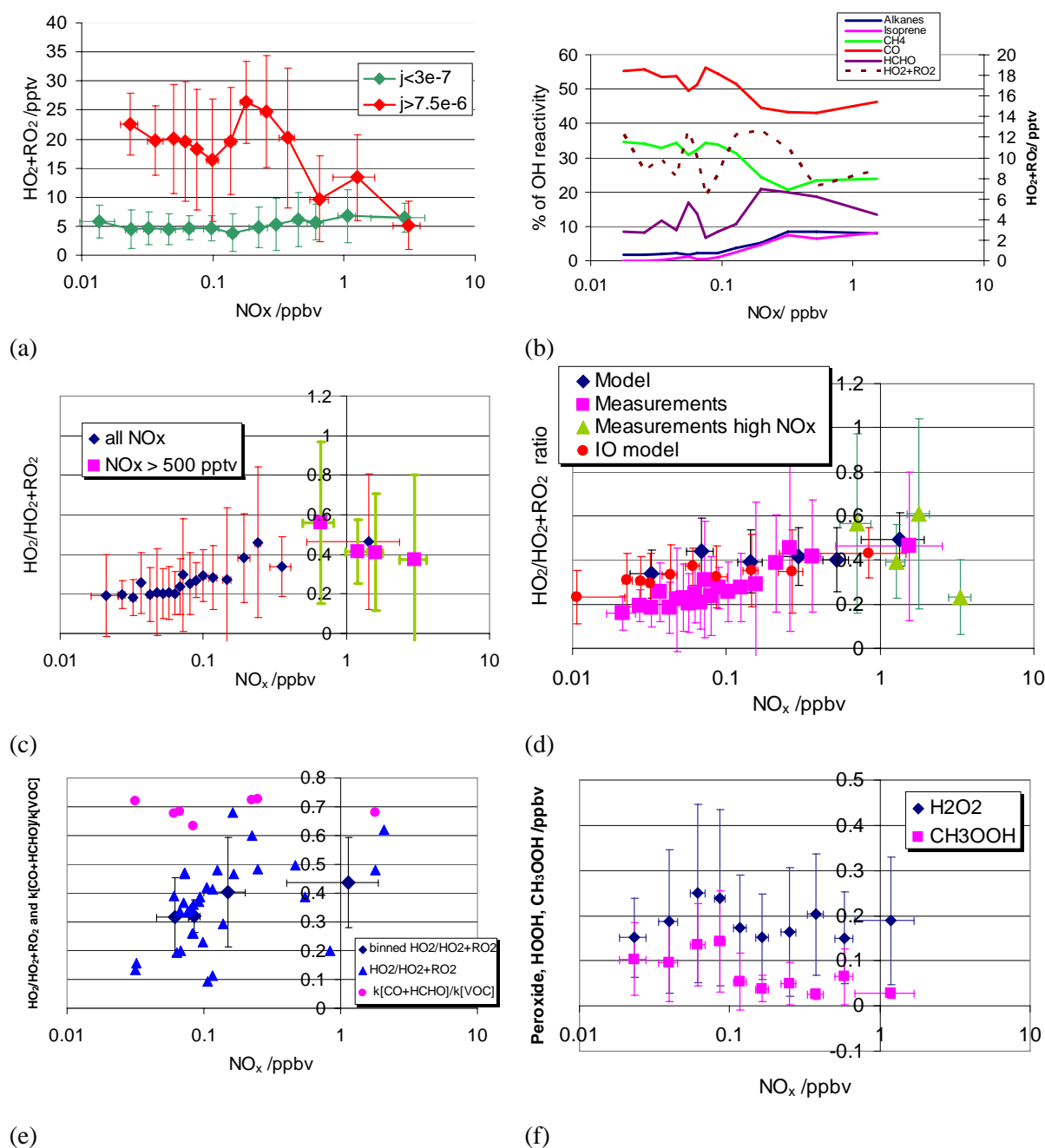
Fig. 8. (a) 10 minute-averaged [HO_2 + \sum RO_2] vs. [NO_x] at two light intensity regimes; (b) Hourly-averaged daylight (06:00–19:00 UT) percentage contribution to OH reactivities for VOCs, CO and [HO_2 + \sum RO_2] vs. [NO_x] ; (c) HO_2 / (HO_2 + \sum RO_2) vs. [NO_x] : 15 minute-averaged data with values at [NO_x] > 500 pptv in smaller bins; (d) Measured and modelled HO_2 / (HO_2 + \sum RO_2) ratios vs. [NO_x] for hourly-averages (Model days: 1, 2, 9, 10, 15–22, 31 August and 1 September – model runs both full-oxy with and without halogens (see Table 4)); (e) Hourly-averaged HO_2 / (HO_2 + \sum RO_2) and \phi(CO+HCHO) vs. [NO_x] ; (f) Hourly-averaged [peroxide] vs. [NO_x] ; for details of binning procedure, see text.
