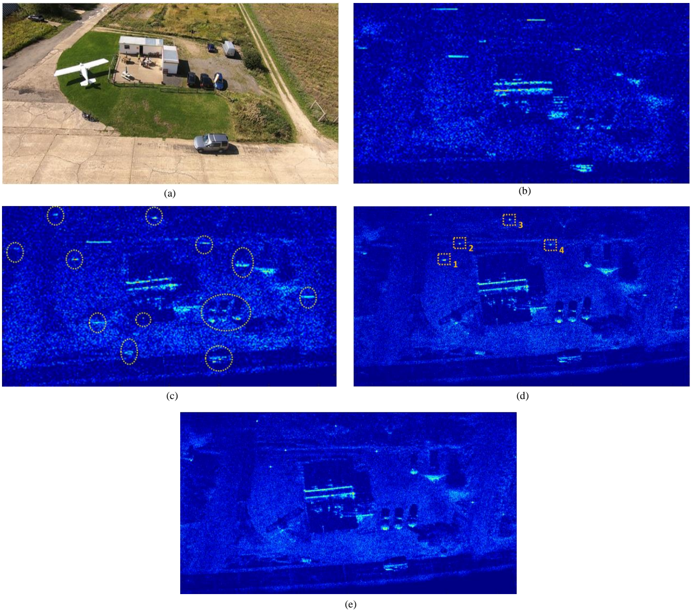
Fig. 12. (a) A picture from the experimentation site. (b) The image without MoCo. (c) The image with MoCo using GPS data. (d) The image after the RCMC step. (e) The final image after azimuth and range blocks based MoCo.
