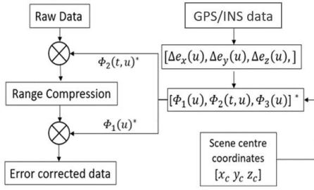
Fig. 4. GPS/INS based MoCo.
