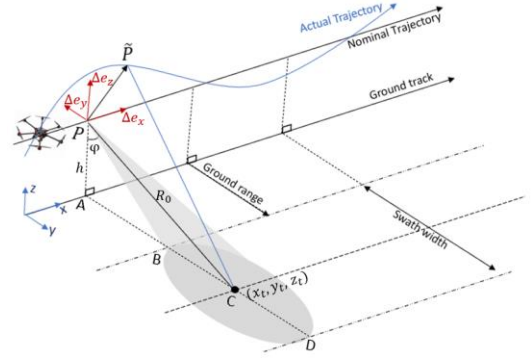
Fig. 1. Drone-borne SAR image geometry
