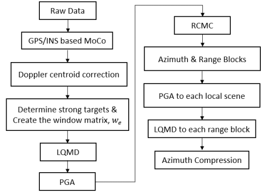
Fig. 3. The flow chart of the algorithm.
