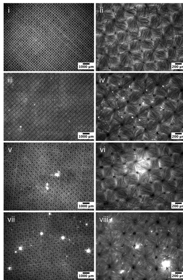
Fig. 3 Fluorescent micrographs of (i–ii) blank WFK10A cotton, and the cotton samples exposed to 0.3% PDMS emulsion prepared using (iii–iv) 10^3 cSt PDMS; (v–vi) 10^4 cSt PDMS, and (vii–viii) 10^5 cSt PDMS. The bright regions correspond to the presence of the surface deposited PDMS.
