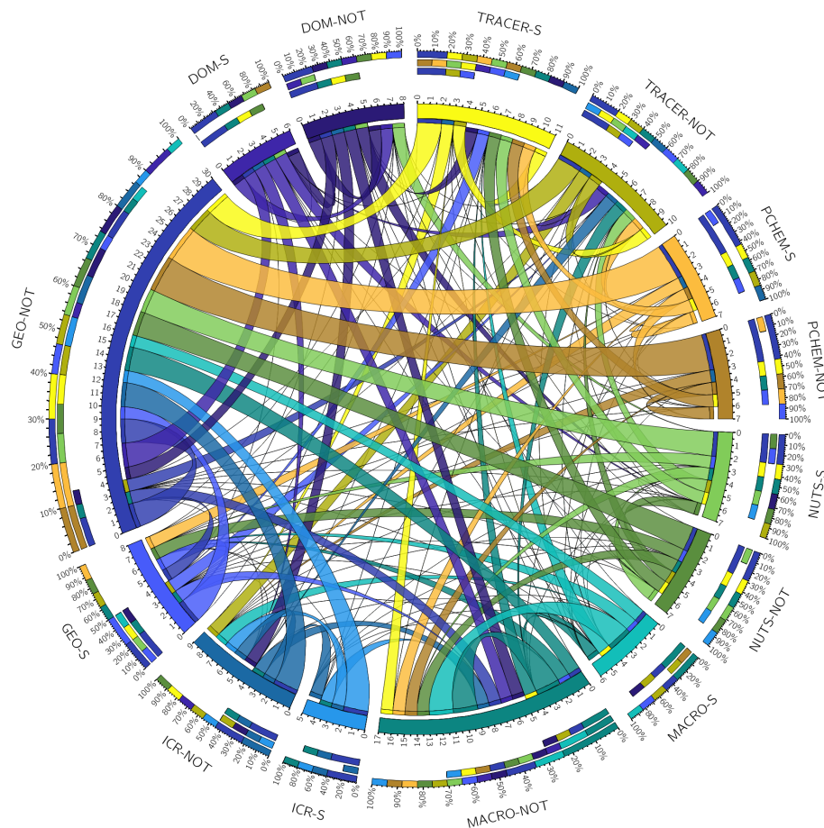
FIGURE 2 Information flow within and among subgroups of variables commonly used as measures of river corridor dynamics based on the suite of support vector machine regression (SVMRs) constructed for each variable (Section 3.3.1). The variables included in the seven subgroups (PCHEM = physical chemistry; GEO = geologic setting; NUTS = nutrients; ICR = metabolomics; DOM = dissolved organic matter; MACRO = macroinvertebrate; TRACER = stream solute tracer; variables in each grouping are detailed in Ward (2021)) are further organized by those with spatial structure ('-S') and without spatial structure ('-NOT'). Each subgroup is represented by a different colour to enable visualization of interactions with other subgroups, with the colour of each 'ribbon' denoting the origin of information (i.e., the subgroup from which information flows). The width of each 'ribbon' denotes the relative frequency of interaction between variable groups. The three 'rings' around the outside of the plot represent information flow between subgroups as Inner Ring: destination(s) of information from each subgroup (i.e., answers the question 'which other subgroups used information from this subgroup?'; colloquially the 'outflows' of information from one subgroup to another). These are the independent variables requires as inputs to make predictions of dependent variables in other groups. Middle Ring: the source(s) of information to a subgroup (i.e., answers the question 'which variable informed relationship using to predict variables in a given subgroup?'; colloquially the 'inflows' of information to a subgroup). These are the independent variables providing information for predictions of variables within this group. Outer Ring: Scaled, total interactions with other variable groups regardless of directionality (i.e., answers the question 'how related is this subgroup to others in the web of relationships?'). These are the relative magnitudes of direction-independent relationships between subgroups
