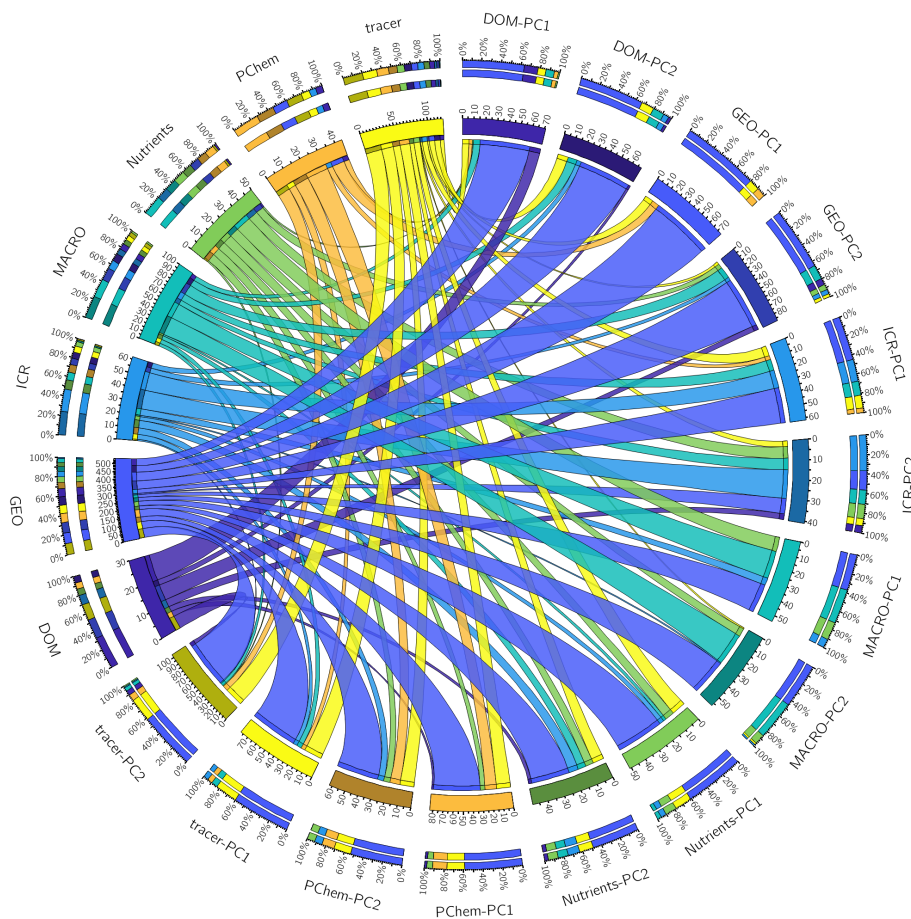
FIGURE 4 Circos plot showing the one-way flow of information from the subgroup PCs (Table 1; labelled ‘XXX-PCY’ where XXX is the subgroup and Y in the PC number) to variables predicted by the suite of SVMRs described in Section 3.3.2. Plot layout and interpretation is identical to that described for Figure 2, except that ‘flows’ of information only originate the PCs (i.e., subgroup PCs have only outflowing and total interactions; middle and outer rings) and only inform variables in the subgroups (i.e., variable subgroups only have inflowing and total interactions; inner and outer rings)
