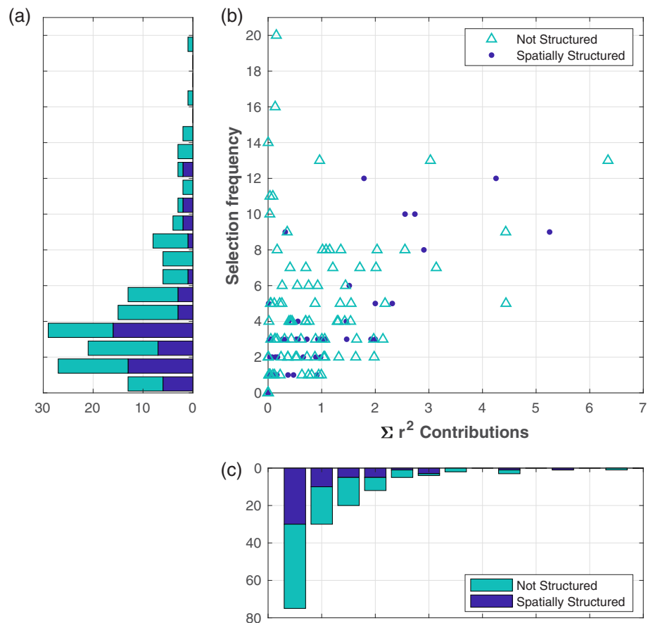
FIGURE 3 Distributions of variable selection frequency and contributions of each variable to improvement in r^2 for all 157 SVRMs constructed on all variables. (a) Histogram of the frequency with which individual variables were selected. (b) Variable selection frequency versus total improvement in r^2 . (c) Histogram of contributions of variables to r^2
