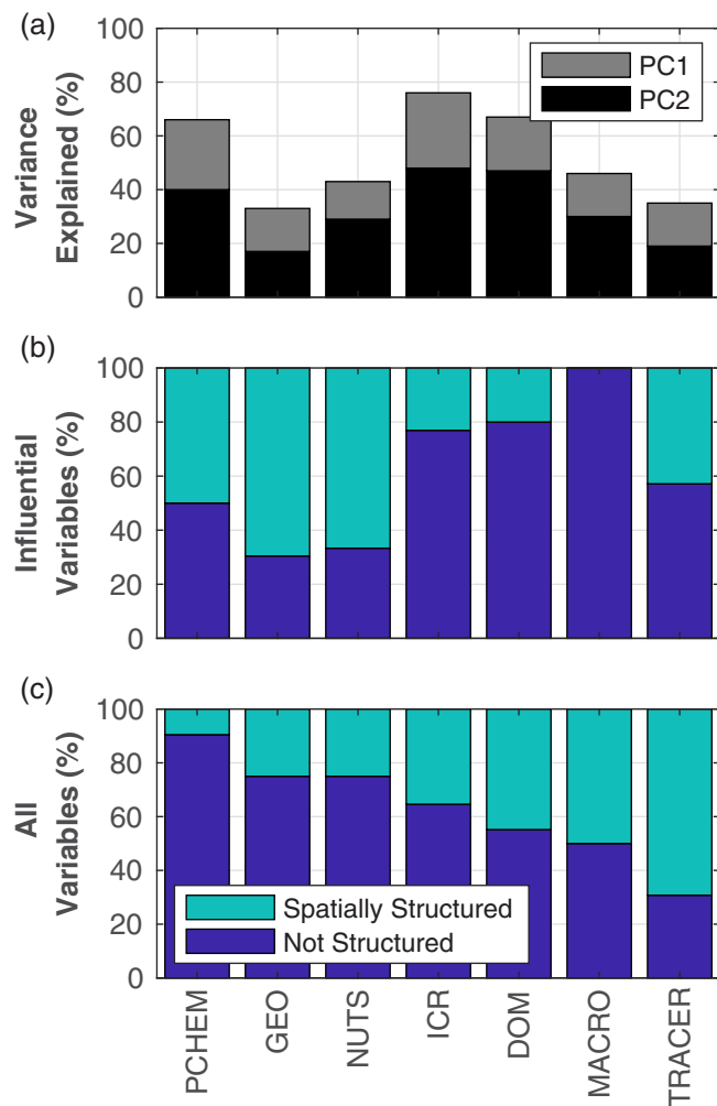
FIGURE 1 (a) Variance in the Andrews river corridor data set explained by PC1 and PC2 for each expert subgroup. (b) Percentage of influential variables (i.e., the variables included in the first two PCs) that do and do not have spatial structure. (c) Percentage of all variables within each subgroup that do and do not have spatial structure
