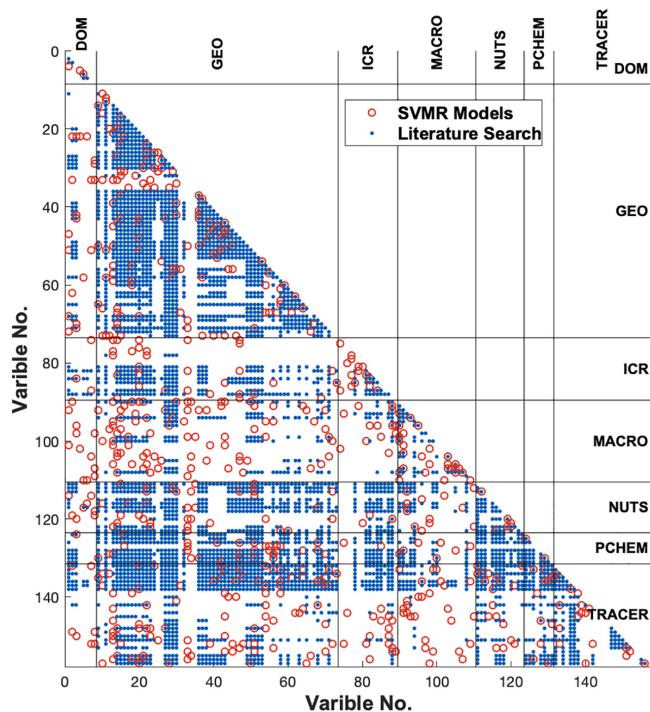
FIGURE 5 Scatterplot showing pairwise study in the literature (blue dots) and identification of a relationship in our support vector machine regression approach (red circles) for all variable pairs. Variable numbers correspond to the order variables are listed in Table S1
