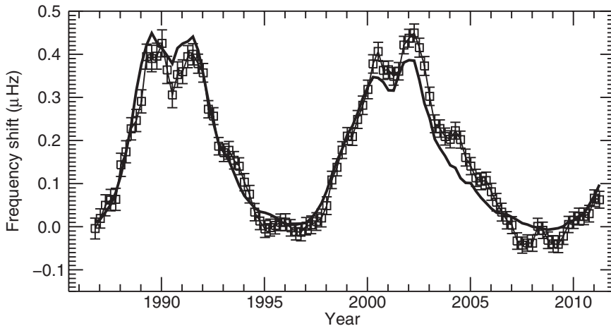
Figure 4. Oscillation frequency shifts in the high frequency band with the 10.7 cm flux overplotted as a thin line. The 10.7 and the frequency shifts are scaled to match in cycle 22
