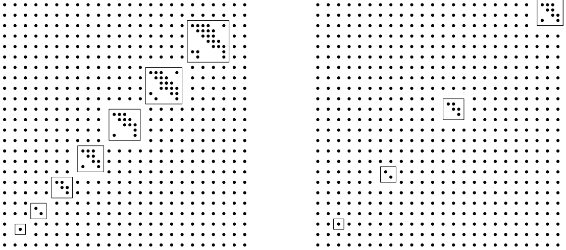
Figure 1: Examples of ‘very different’ separated nets X_1 (left) and X_2 (right). The cubes in (S_k^1) are the same as in (S_k^2) , but the distance of S_k^1 to the origin grows with k much slower than that of S_k^2 .
