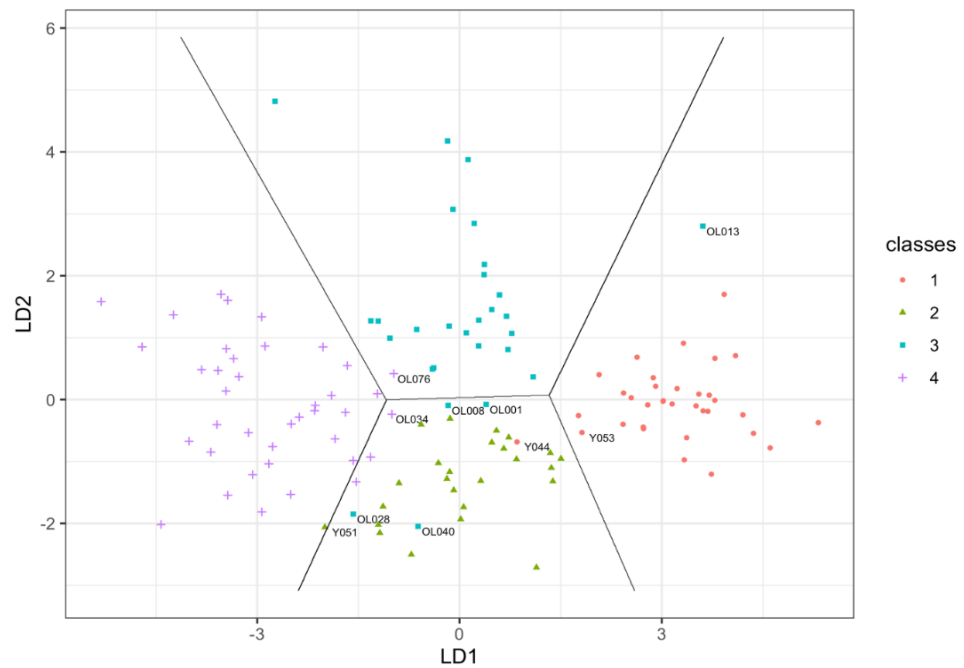
Figure 1. Decision boundaries from the linear discriminant analysis in the two-dimensional subspace spanned by the first two discriminant functions (LD1 and LD2) with misclassified cases labelled. Predicted classes indicated by colour: red; young males, green; young females, blue; older males, lilac; older females.
