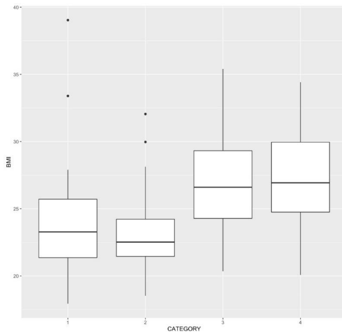
Figure 2. Boxplots of BMI and four categories; 1 = Young male, 2 = Young female, 3 = Older male, 4 = Older female. The whiskers of the boxplots extend to 1.5 times interquartile range for each category. Data beyond the end of the whiskers are plotted individually.
