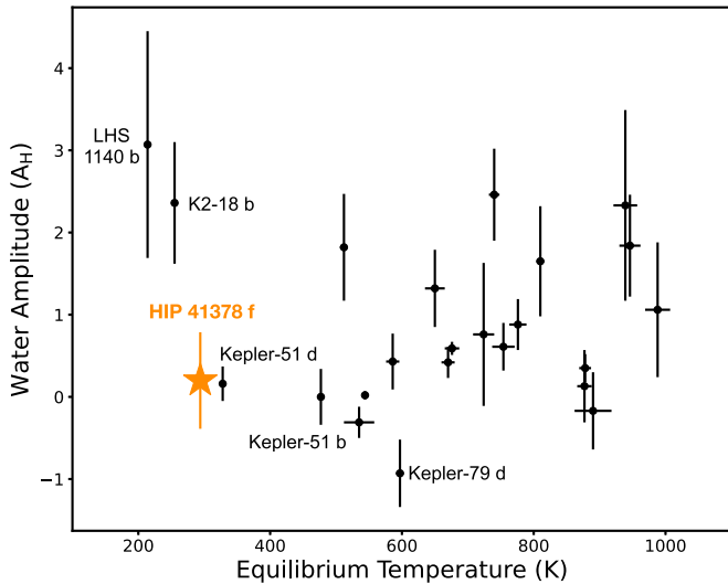
Figure 3. Equilibrium temperature vs. the 1.4 \mu\text{m} \text{H}_2\text{O} feature amplitude ( A_H ) for the cooler ( T_{\text{eq}} < 1000 K) planets sample from Dymont et al. (2021) (points) and HIP 41378 f (orange star). There is no clear trend in A_H with planetary temperature.
