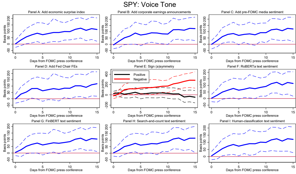
FIGURE 14. ROBUSTNESS CHECKS
