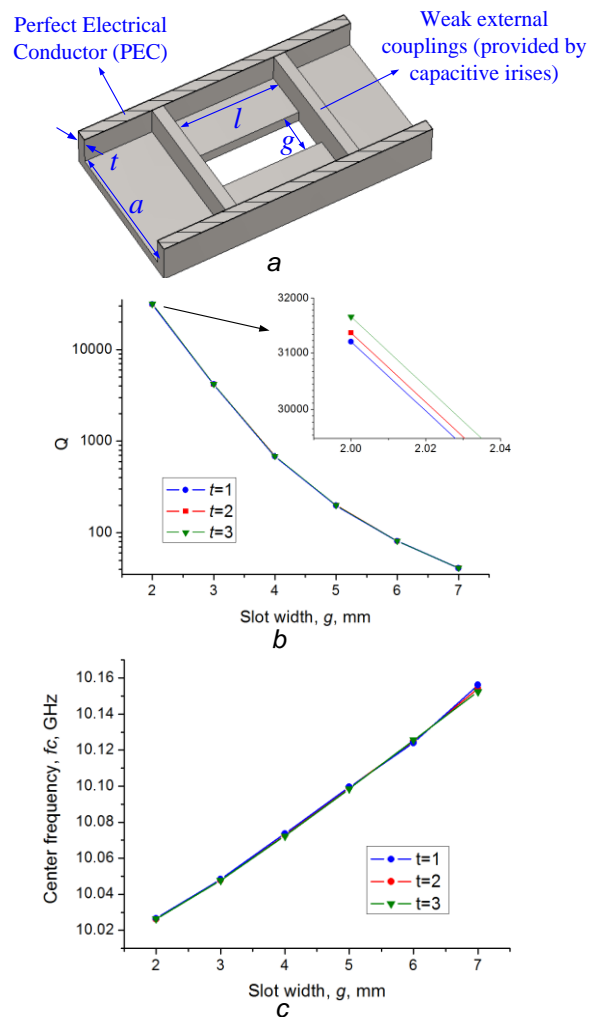
Fig. 2 An X-band TE_{101} cavity resonator with broadside wall slots.
