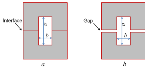
Fig. 1 Illustration of E-plane split waveguide.
