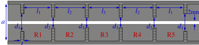
Fig. 3 Configuration of the X-band filter and its dimensions.
