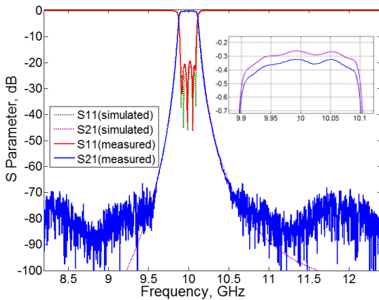
Fig. 5 Measurement (solid lines) and simulation (dashed lines) results of the filter. The insert shows enlarged view of the filter responses over passband. No tuning screws have been used in the measurements.
