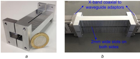
Fig. 4 Photograph of the fabricated X-band filter.
