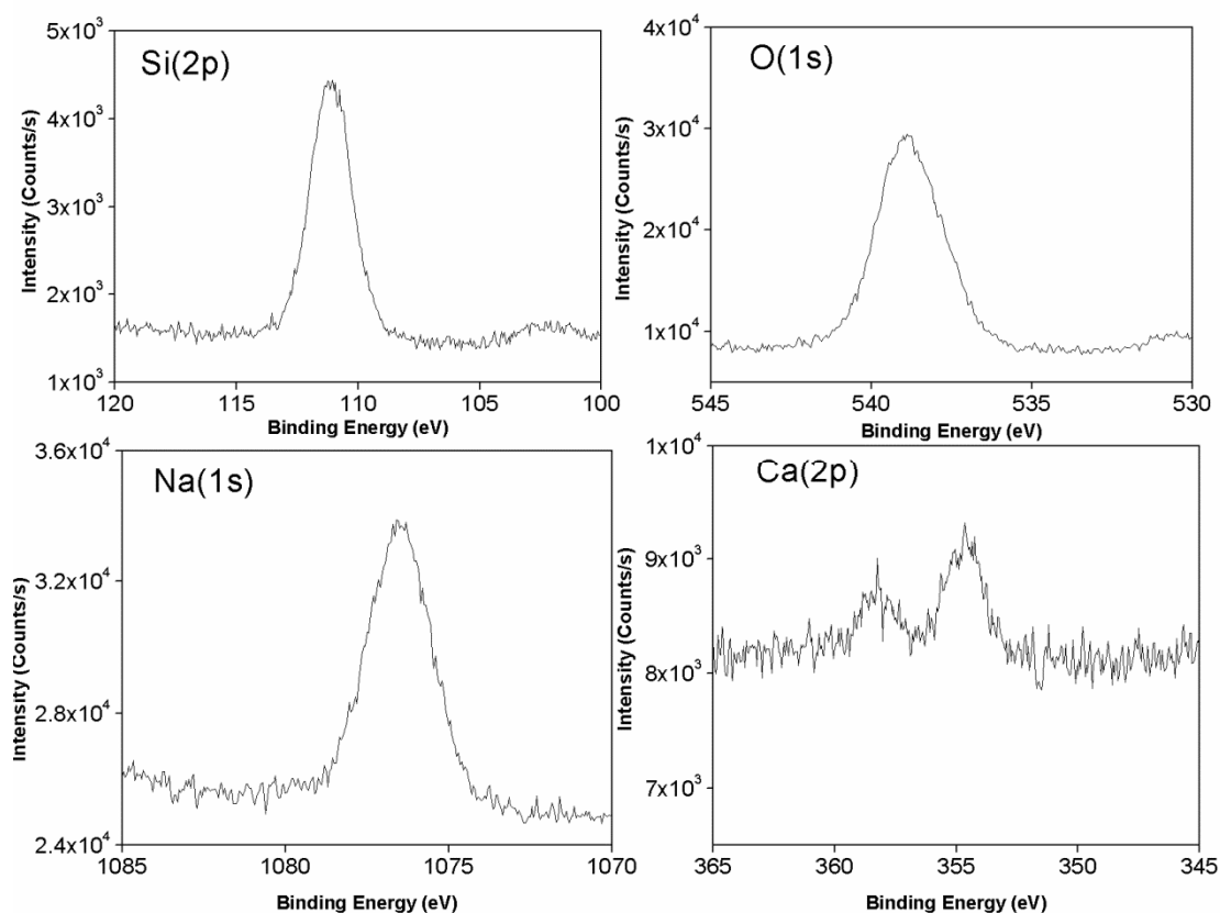
Figure 1 XPS spectra of glass capillary interior (Li et al., 2014)
