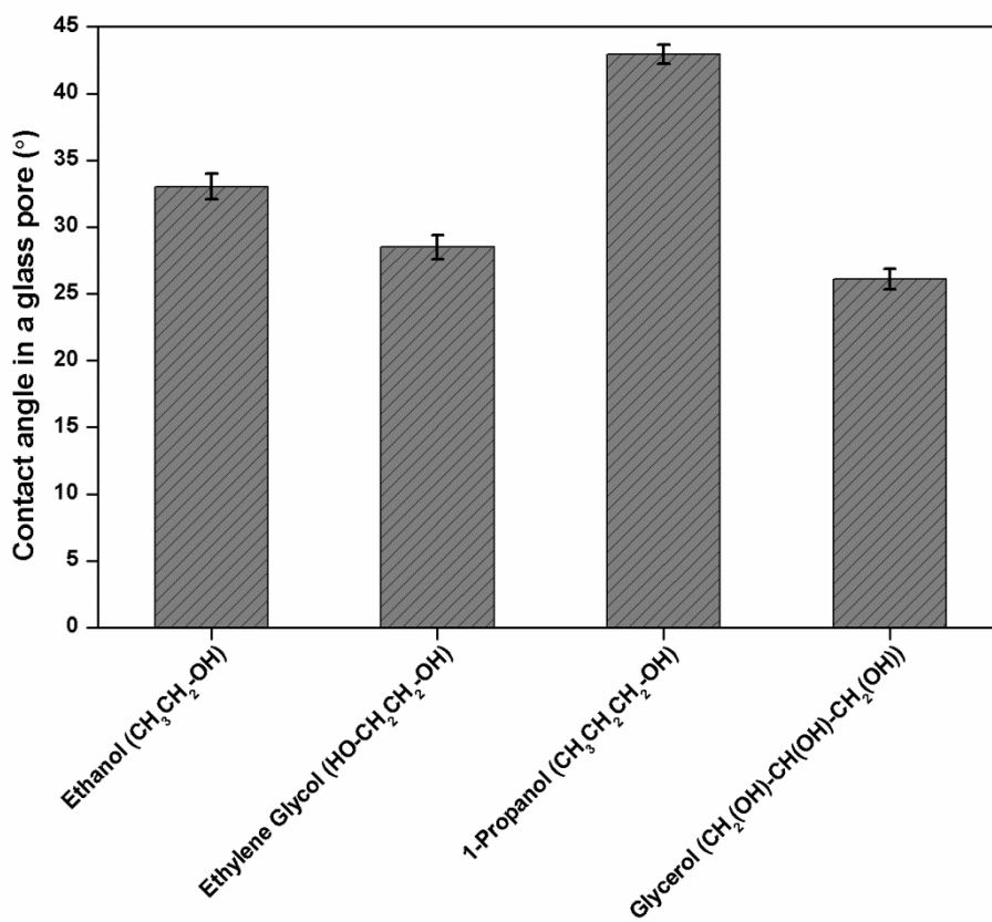
Figure 9 The pore contact angles of ethanol, ethylene glycol, 1-propanol and glycerol
