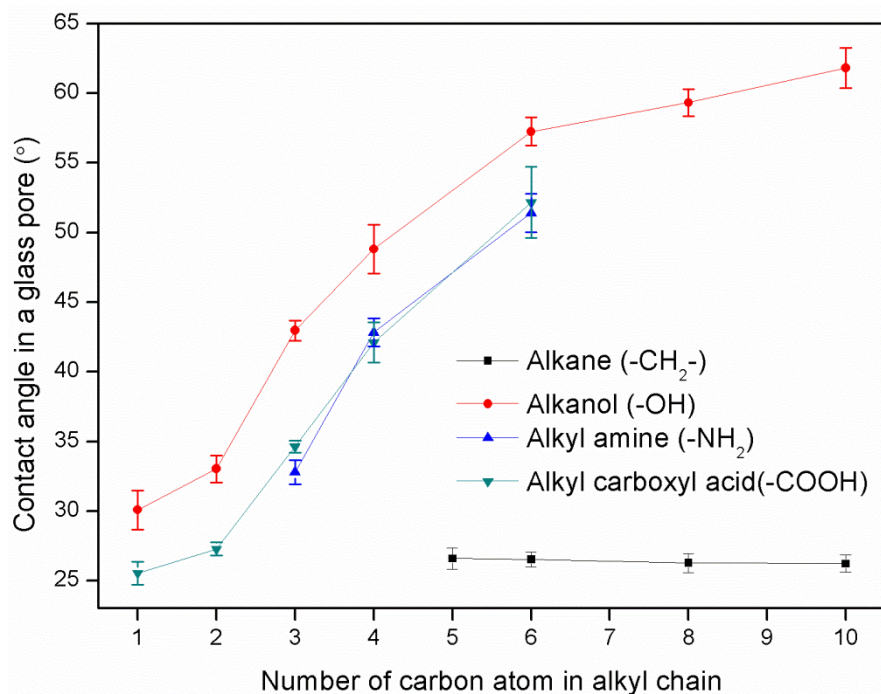
Figure 7 Pore contact angles of alkanes, alkanols, alkylamines and alkyl carboxyl acid with different straight alkyl chain lengths.
