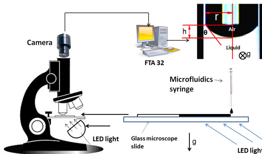
Figure 2 Experimental setup for the study of the contact angle in a capillary. (the vector \mathbf{g} shows the direction of gravity) (Li et al., 2013)
