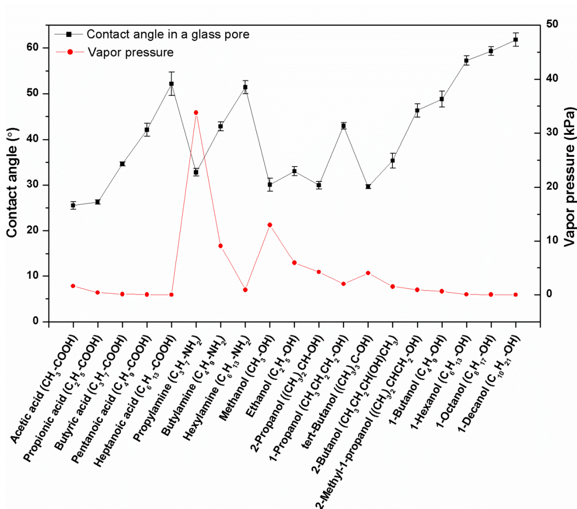
Figure 5 Contact angles in a pore and vapor pressures at 20 °C for all amphiphiles used in this study
