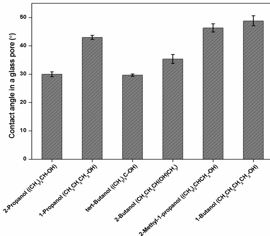
Figure 8 Pore contact angles of structural isomers of 1-propanol and 1-butanol
