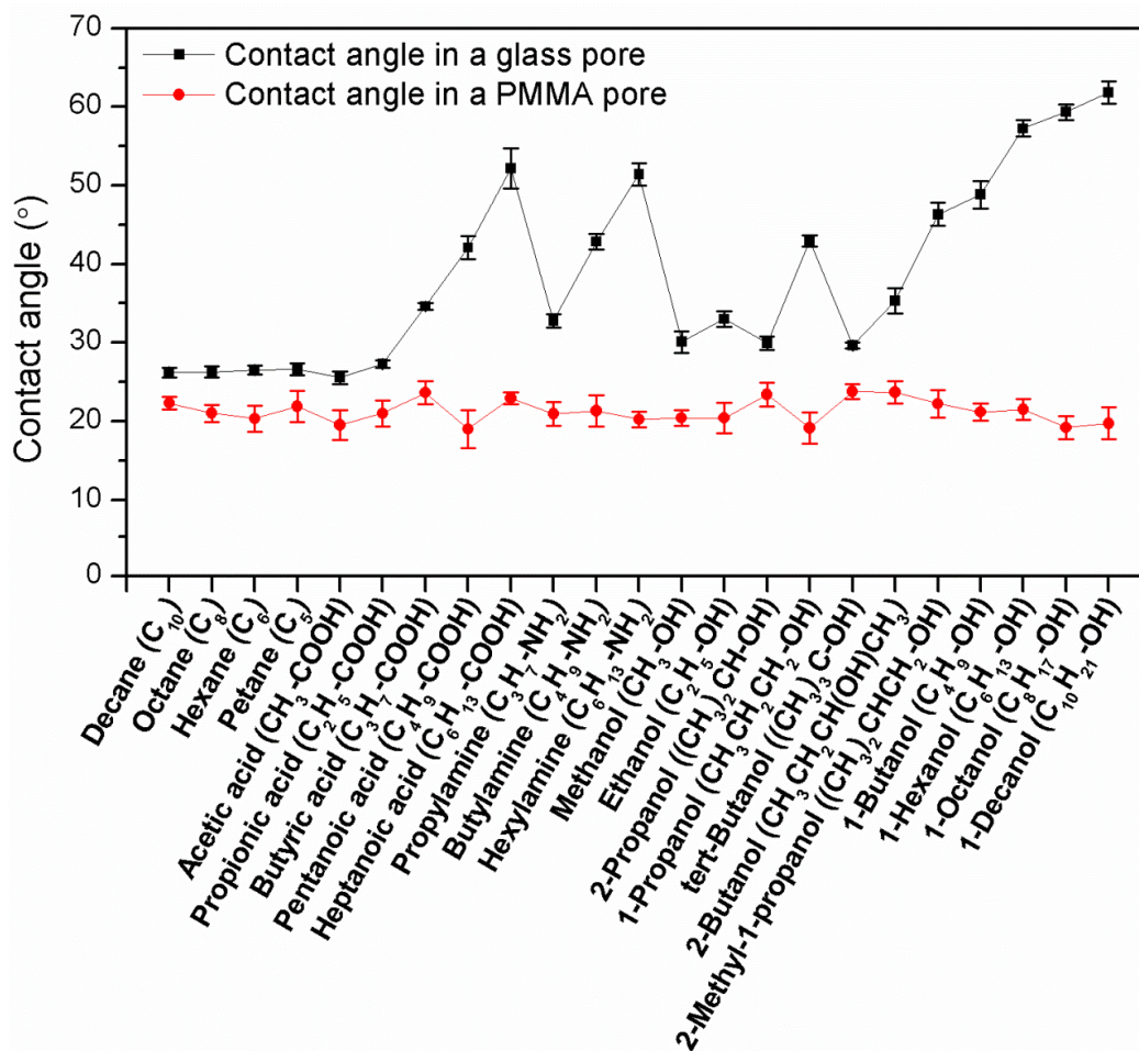
Figure 4 Comparison of contact angles measured in a glass pore and a PMMA pore
