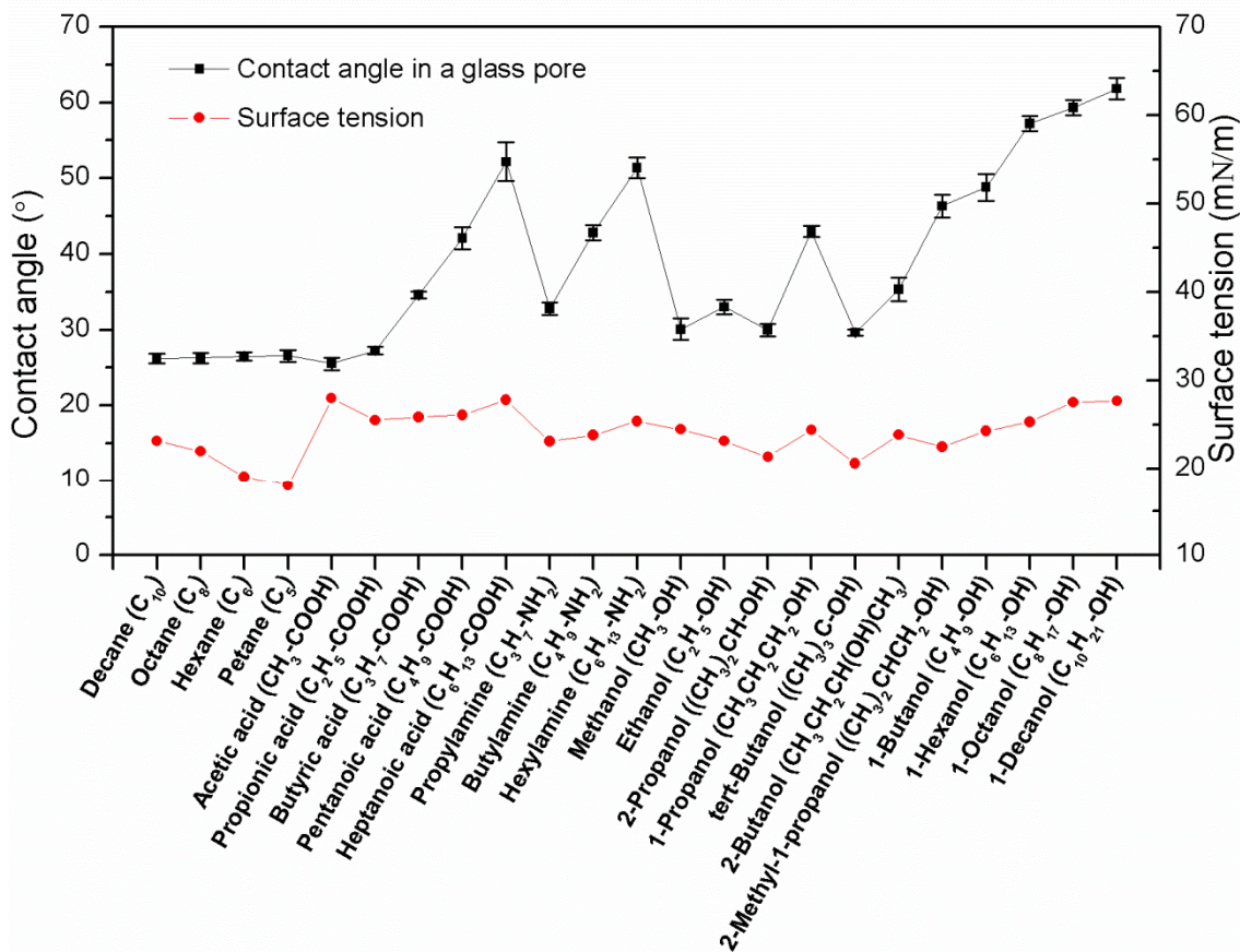
Figure 3 Contact angles in a glass pore and the surface tensions for the organics used in this study
