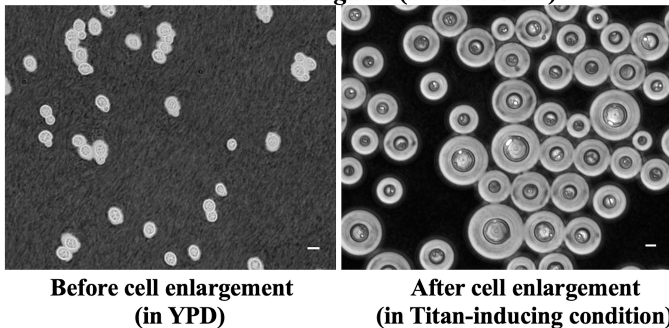
Fig 1. Micrograph showing the budding nature of C. deuterogattii yeast (left panel) vs. titan (right panel) cells [44]. Scale bar = 5 \mu\text{m} .
