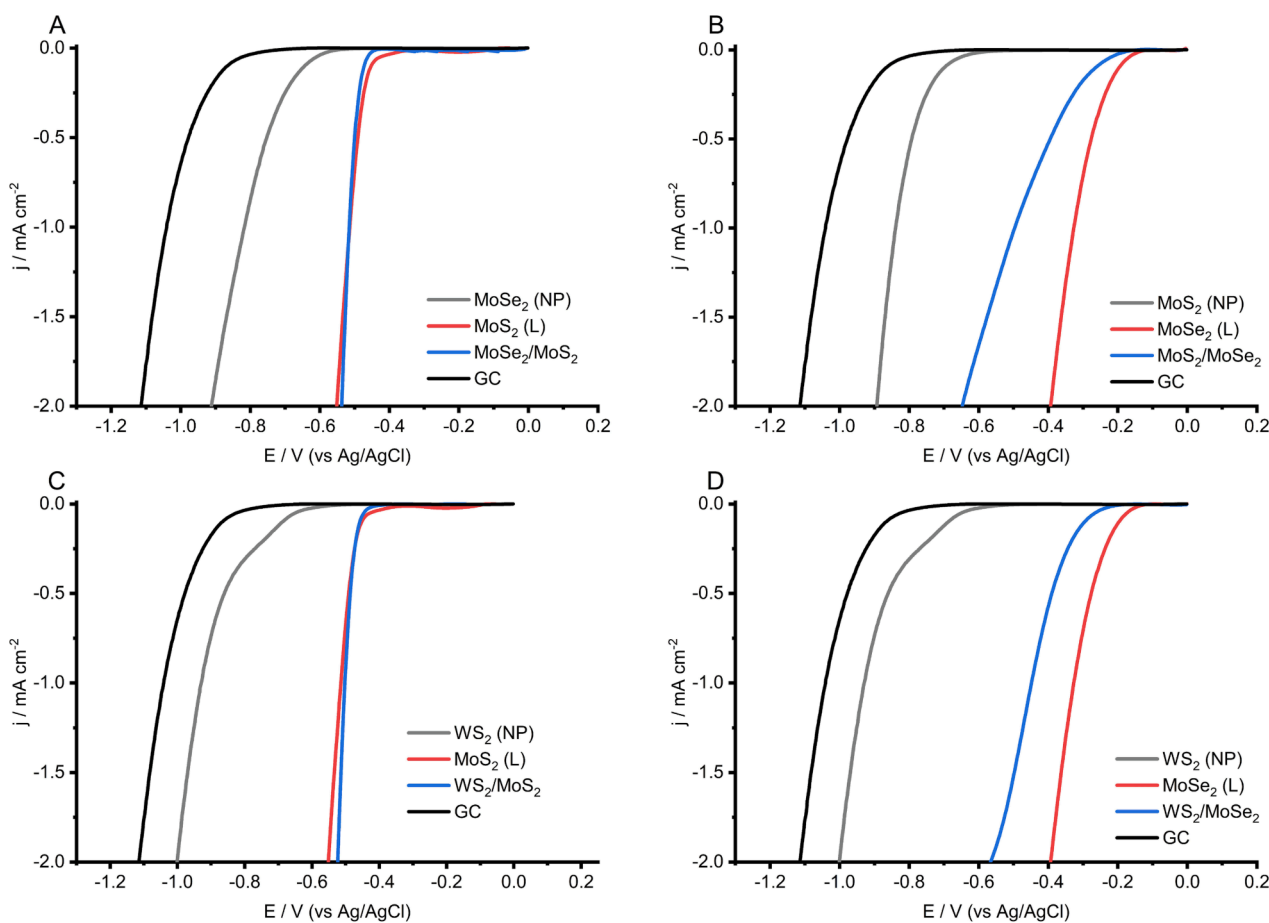
Fig. 3. Linear sweep voltammograms of (A) \text{MoSe}_2/\text{MoS}_2 , (B) \text{MoS}_2/\text{MoSe}_2 , (C) \text{WS}_2/\text{MoS}_2 and (D) \text{WS}_2/\text{MoSe}_2 heterolayers as electrocatalysts for the hydrogen evolution reaction in comparison to the TMDs that make them up. This was done in a solution of 10 \text{ mM H}_2\text{SO}_4 and 0.1 \text{ M K}_2\text{SO}_4 at voltage scan rate of 20 \text{ mV s}^{-1} for all the scans.
