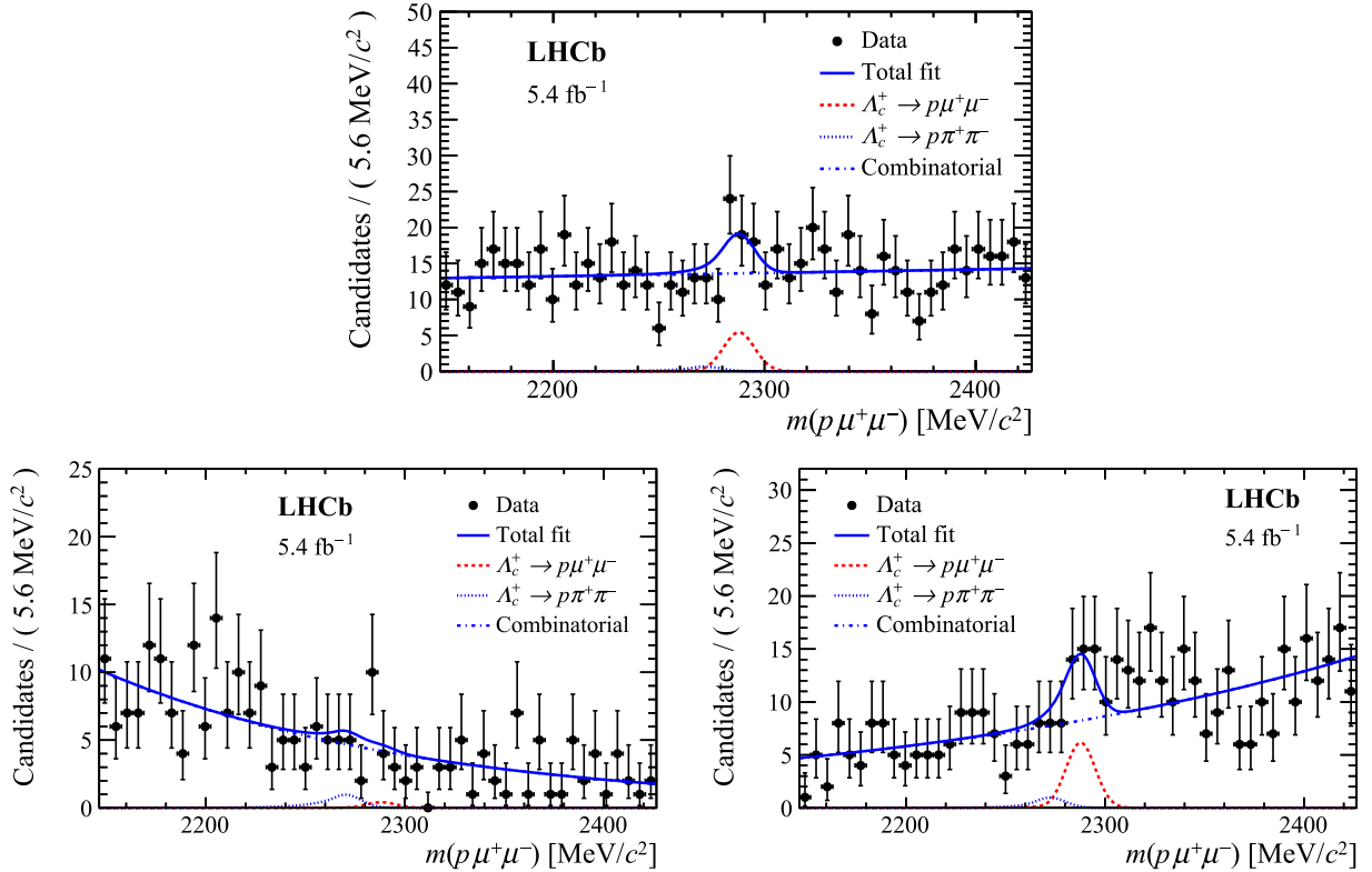
FIG. 1. Distributions of p\mu^+\mu^- invariant mass for (top) signal , (bottom left) low- m and (bottom right) high- m regions. The results of the fit are overlaid.
