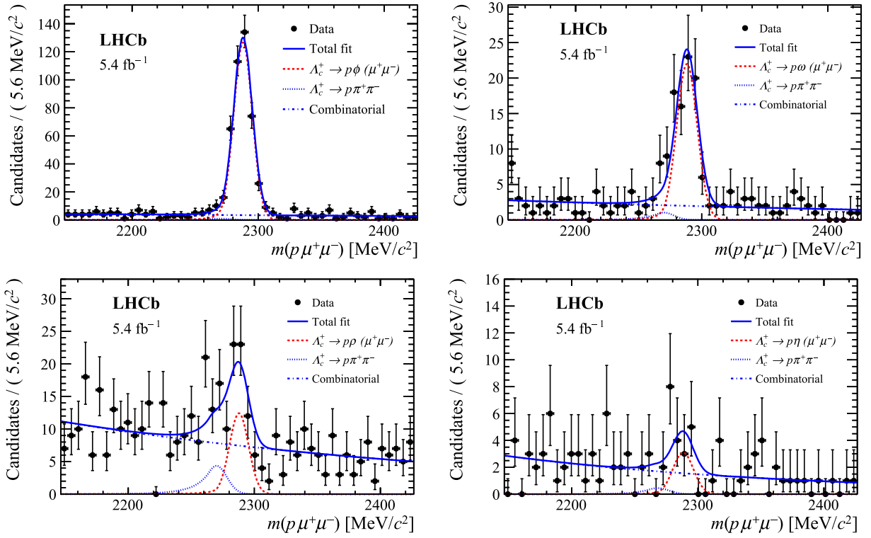
FIG. 2. Distributions of p\mu^+\mu^- invariant mass for (top left) \phi , (top right) \omega , (bottom left) \rho and (bottom right) \eta regions. The results of the fit are overlaid.
