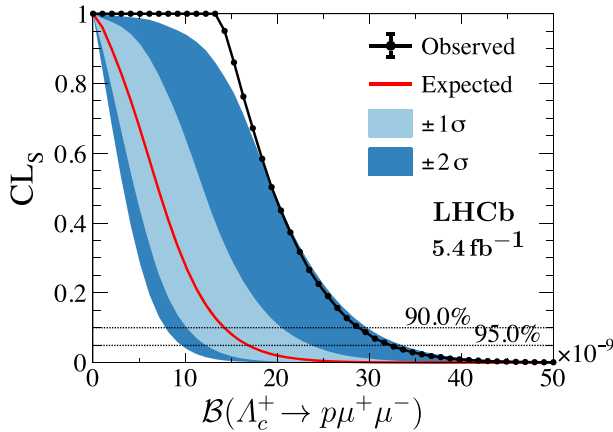
FIG. 3. Observed and expected (background only hypothesis) limits for \Lambda_c^+ \rightarrow p\mu^+\mu^- branching fraction.
