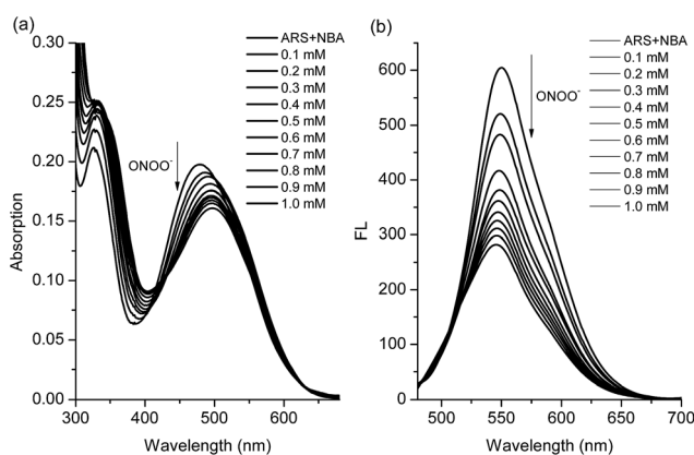
Fig. 3 (a) UV-Vis titration and (b) fluorescence titration ( \lambda_{\text{ex}} = 460 \text{ nm} ) for ARS–NBA (ARS, 50 \mu\text{M} ; NBA, 200 \mu\text{M} ) in the presence of various concentrations of \text{ONOO}^- (0–1 mM). The data was obtained in 52.1% MeOH/ \text{H}_2\text{O} PBS buffer (pH 8.10) at 25 ^\circ\text{C} .
