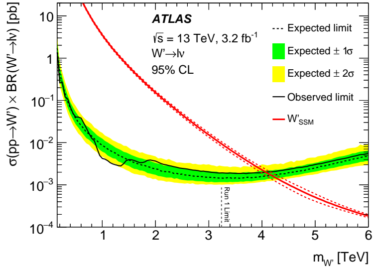
Figure 3: Median expected (dashed black line) and observed (solid black line) 95% CL upper limits on cross-section times branching ratio ( \sigma \times B ) in the combined channel, along with predicted \sigma \times B for W'_{SSM} production (red line). Uncertainties in \sigma \times B from the PDF, \alpha_S and scale are shown as a red-dashed line. The bands for 68% (green) and 95% (yellow) confidence intervals are also shown. The vertical dashed line indicates the mass limit of the 8 TeV data analysis [2].
