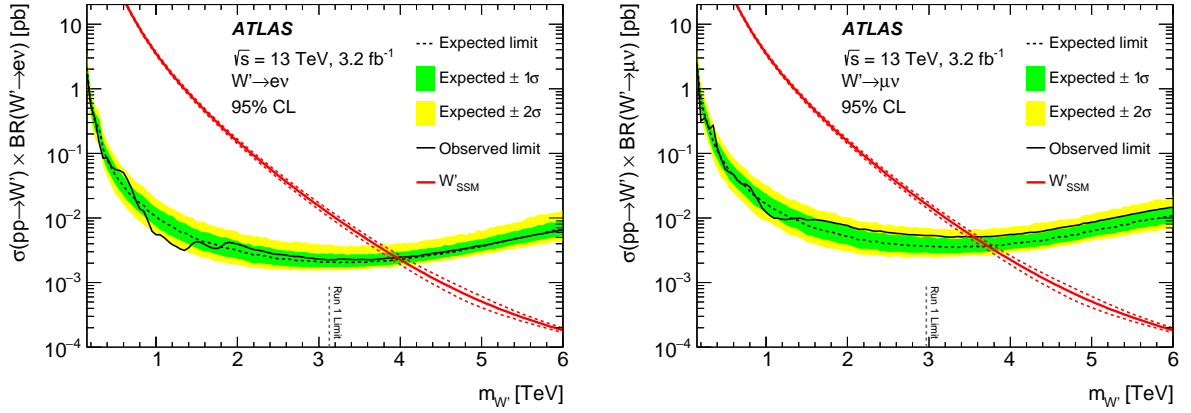
Figure 2: Median expected (dashed black line) and observed (solid black line) 95% CL upper limits on cross-section times branching ratio ( \sigma \times B ) in the electron (left) and muon (right) channels. The bands for 68% (green) and 95% (yellow) confidence intervals are also shown. The predicted \sigma \times B for W'_{SSM} production is shown as a red solid line. Uncertainties in \sigma \times B from the PDF, \alpha_S and scale are shown as a red-dashed line. The vertical dashed line indicates the mass limit of the 8 TeV data analysis [2].
