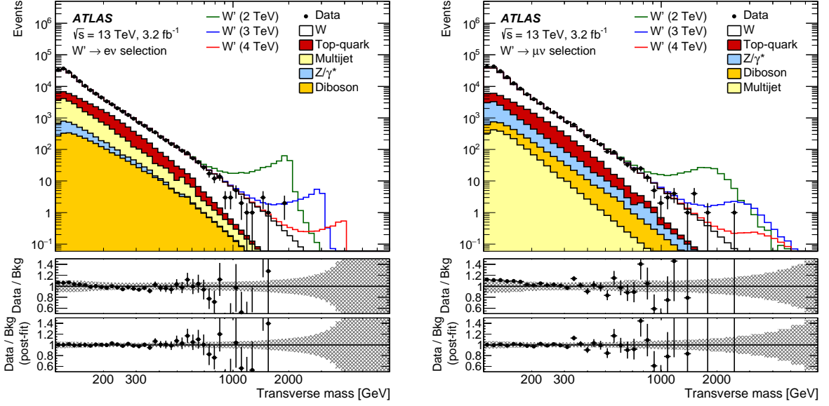
Figure 1: Transverse mass distributions for events satisfying all selection criteria in the electron (left) and muon (right) channels. The distributions are compared to the stacked sum of all expected backgrounds, with three selected W'_{\text{SSM}} signals overlaid. The bin width is constant in \log m_T . The middle panels show the ratio of the data to the expected background. The lower panels show the ratio of the data to the adjusted expected background (“post-fit”) that results from the statistical analysis. The bands in the ratio plots indicate the sum in quadrature of the systematic uncertainties.
