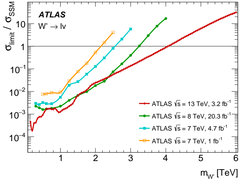
Figure 4: Normalised cross-section limits ( \sigma_{\text{limit}}/\sigma_{\text{SSM}} ) for W' bosons as a function of mass for this analysis and from previous ATLAS searches [2, 39, 40]. The cross-section calculations assume the W' has the same couplings as the SM W boson. The region above each curve is excluded at 95% CL.
