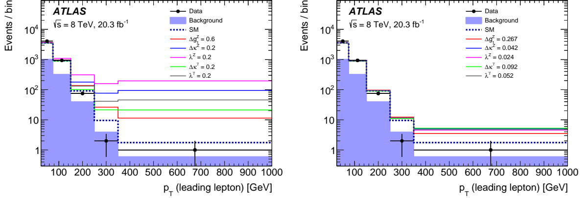
Figure 11: The leading lepton transverse momentum, p_T^{\text{lead}} , for \mu e final states is compared for data and MC-generated events using different arbitrary values for aTGC parameters (left). The detector-level distributions are shown using values of aTGC parameters corresponding to the upper bounds of the observed 95% confidence interval (right). The aTGC parameters are defined in the no constraints scenario, and the form-factor scale is set to infinity. The next-to-leading-order EWK correction scale factors from Table 10 have been applied here. Except for the anomalous coupling parameter under study, all others are set to zero.
