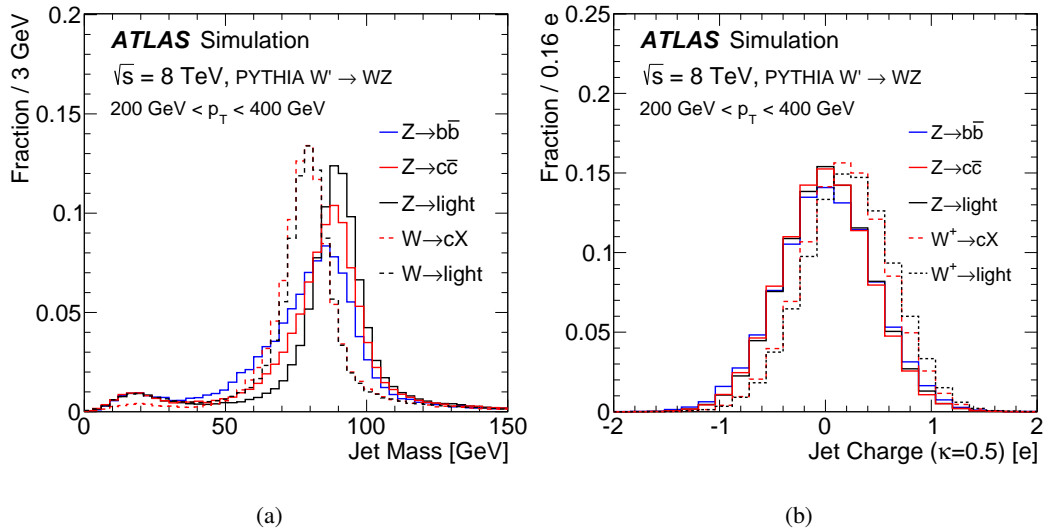
Figure 5: (a) The jet mass p(M|\mathcal{F}, V) and (b) jet charge p(Q|\mathcal{F}, V) templates conditioned on the flavour \mathcal{F} of the boson V decay for jets with 200 \text{ GeV} < p_T < 400 \text{ GeV} . The solid lines are for Z boson decays and the dashed lines are for W boson decays.
