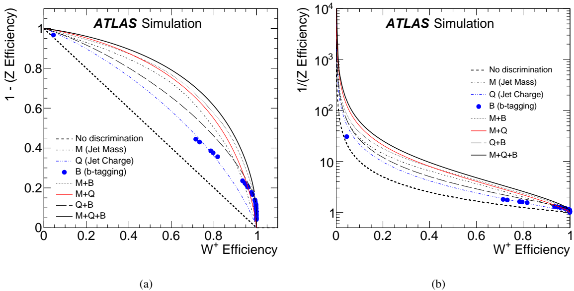
Figure 8: The tradeoff between W^+ \text{ efficiency} and (a) 1 - (Z \text{ efficiency}) or (b) 1/(Z \text{ efficiency}) on (a) a linear scale and (b) a logarithmic scale. Each curve is constructed by placing thresholds on the likelihood constructed from the inputs indicated in the legend. Since the b -tagging discriminant is binned in efficiency, there are only discrete operating points for the tagger built only from B .
