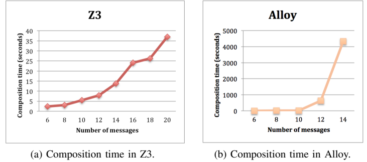
Figure 6: Composition time in Z3 and Alloy
