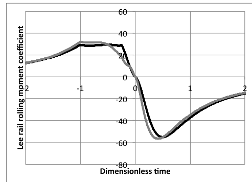
b) Dynamic effects on rolling moment coefficient (black line – no correction; grey line – with correction)
