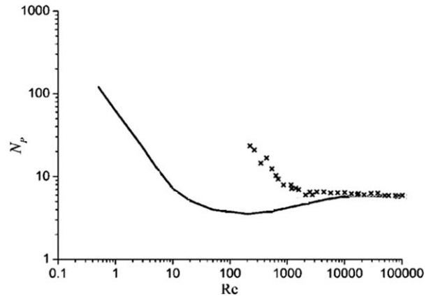
Figure 13. Measured power numbers for Rushton turbine compared to standard values (24).
